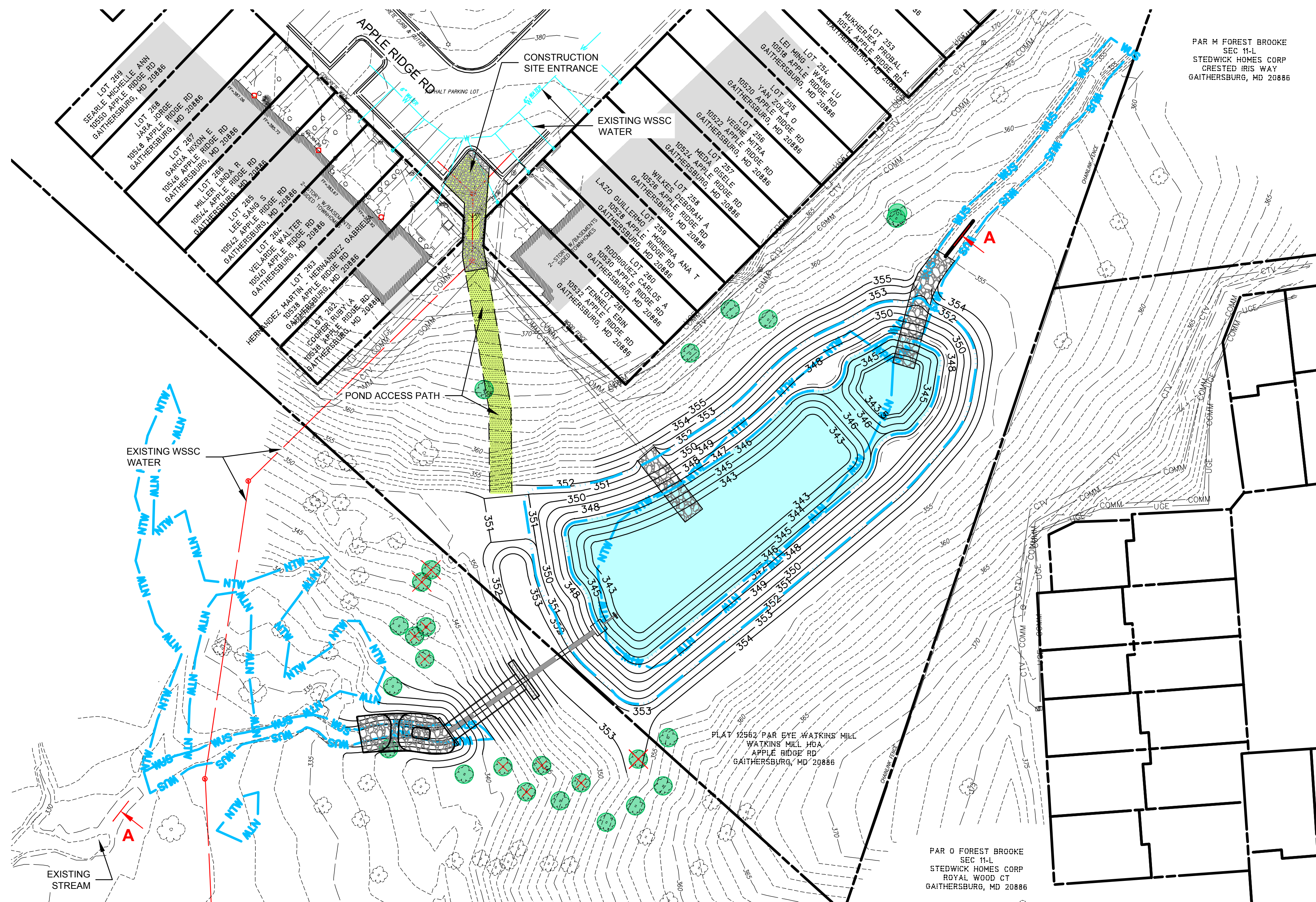
PLAN VIEW
