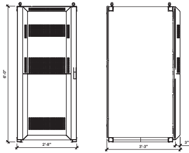
AT&T NETSURE 512 DC POWER CABINET SPECS SCALE: 3/4"=1'-0"
