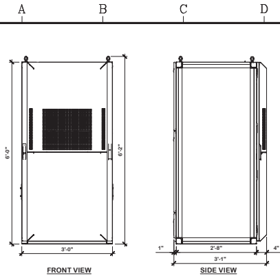
AT&T NETXTEND BATTERY CABINET SPECS SCALE: 3/4"=1'-0"
