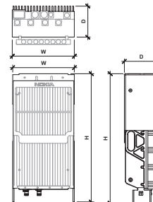
NOKIA AIRSCALE DUAL RRH 4T4R B25/66 480W AHFII DETAIL NOT TO SCALE
