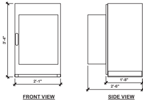
AT&T FLX21-250 EQUIPMENT CABINET SPECS SCALE: 3/4"=1'-0"
