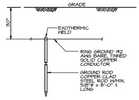
DETAIL - GROUND ROD NO SCALE
