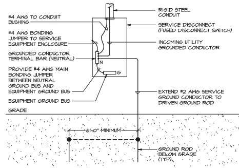
DETAIL - TYPICAL ELECTRIC SERVICE GROUNDING ELECTRODE NO SCALE
