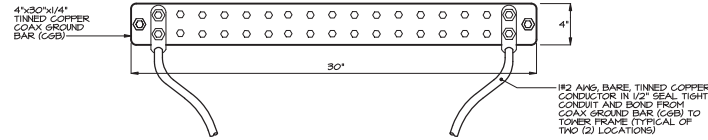
DETAIL - NEW COAX GROUND BAR NO SCALE
