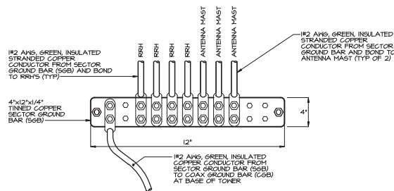
DETAIL - ANTENNA SECTOR GROUND BAR NO SCALE
