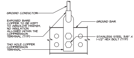
DETAIL - DOUBLE LUG CONNECTION NO SCALE
