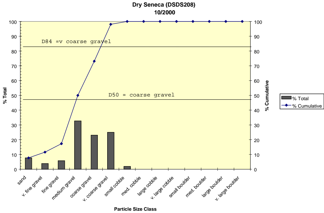
Figure 12. Particle size class distribution for station DSDS208.
