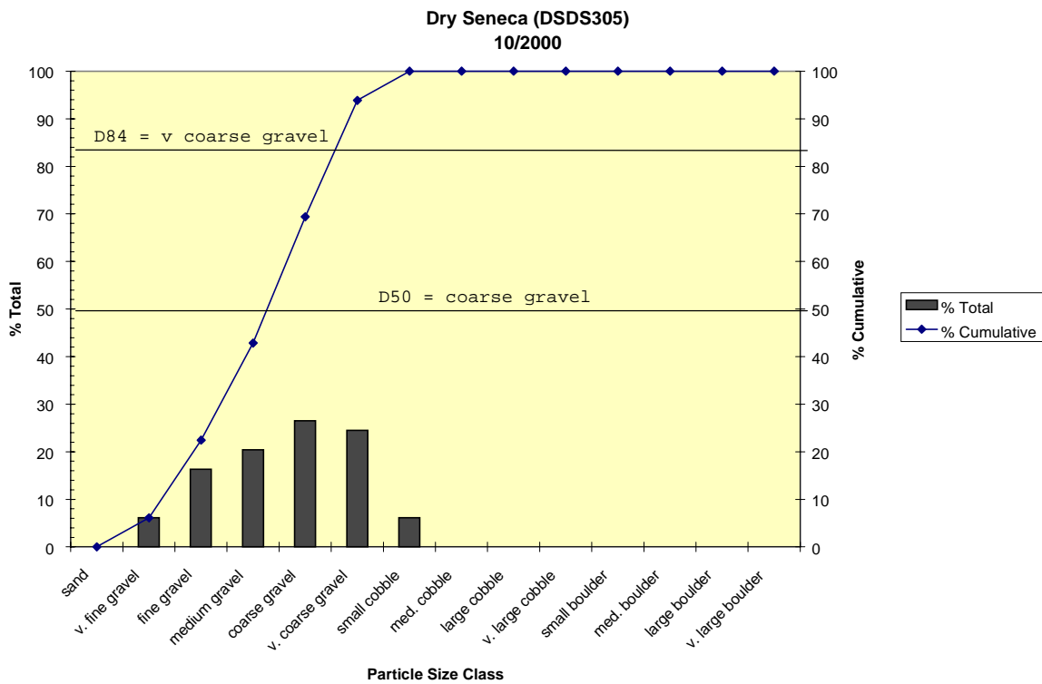
Figure 13. Particle size class distribution for station DSDS305
