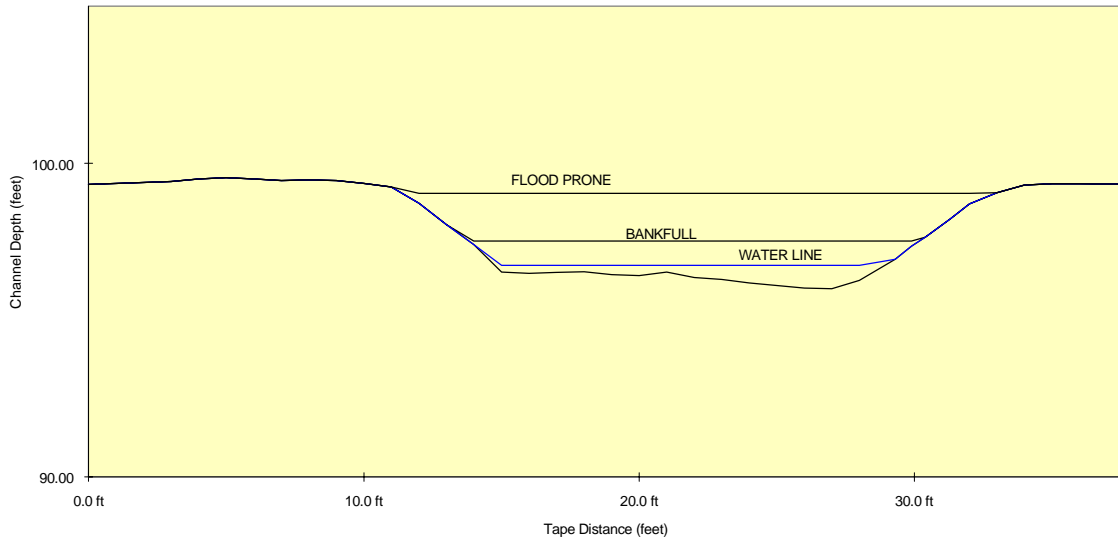
Figure 10. Stream cross section from station DSDS305
