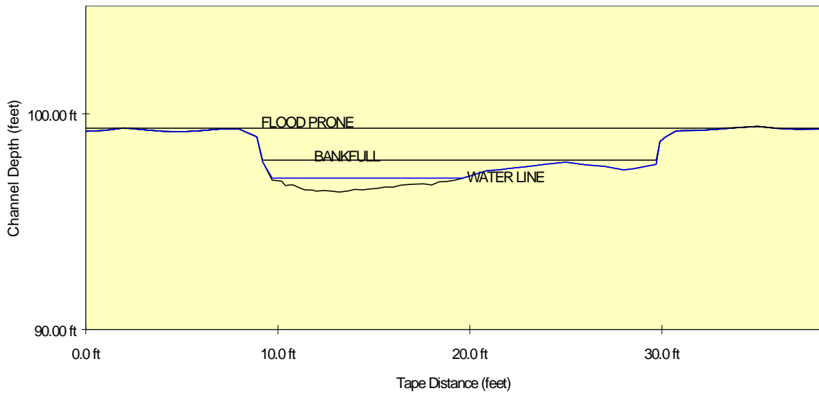
Figure 11. Stream cross section from station DSDS306.
