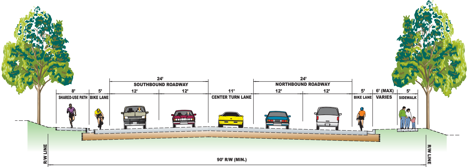
SNOUFFER SCHOOL ROAD TYPICAL SECTION FROM WOODFIELD ROAD (MD 124) TO GOSHEN ROAD *NOTE: SECTION SHOWN IS PROPOSED BY OTHERS
