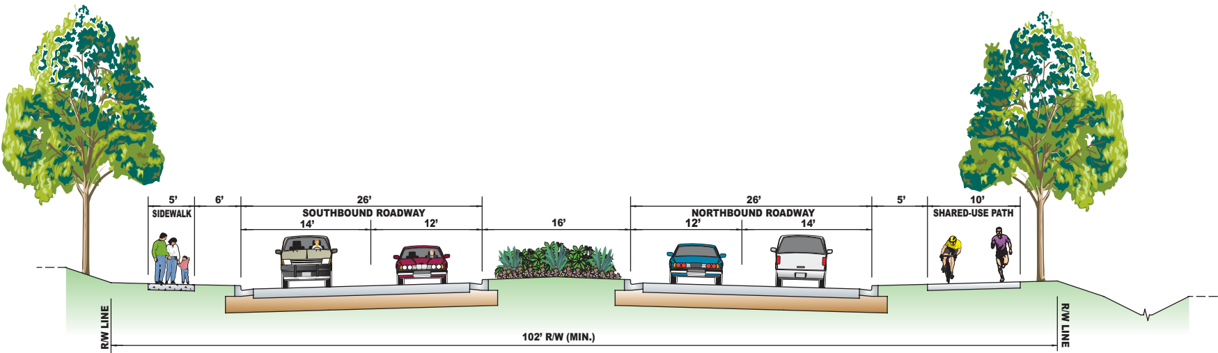
WIGHTMAN ROAD / BRINK ROAD TYPICAL SECTION FROM GOSHEN ROAD TO RIDGE ROAD (MD 27)
