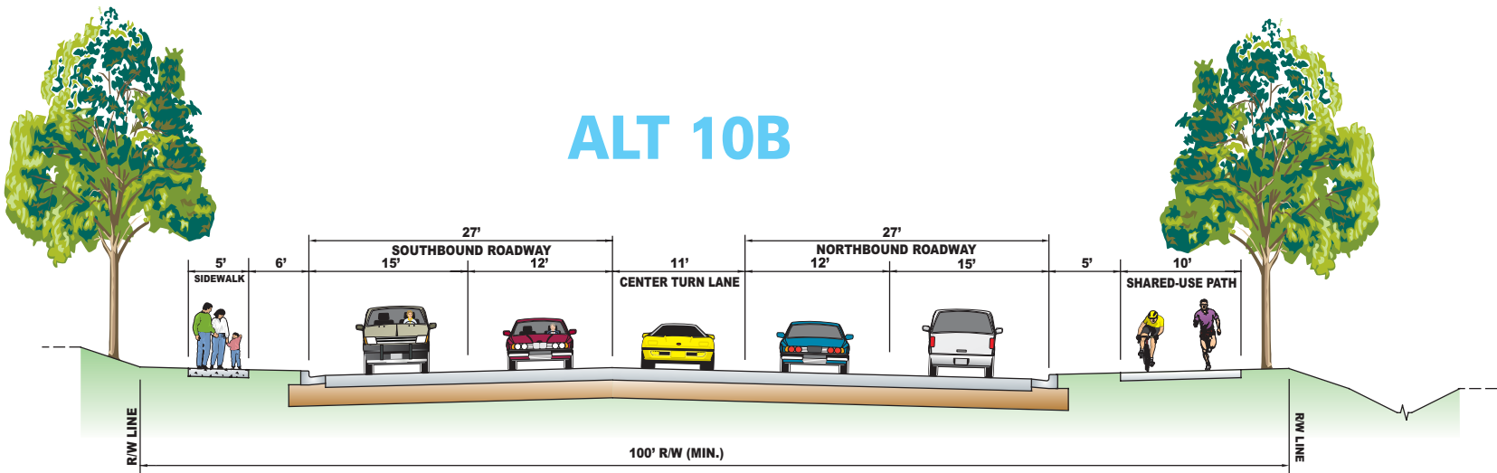
MUNCASTER MILL ROAD (MD 115) TYPICAL SECTION FROM SHADY GROVE ROAD / AIRPARK ROAD TO WOODFIELD ROAD (MD 124)
