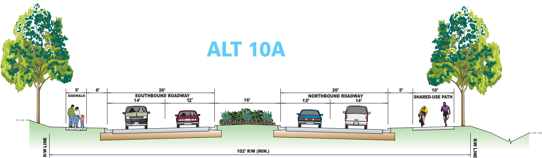
MUNCASTER MILL ROAD (MD 115) / SNOUFFER SCHOOL ROAD / WIGHTMAN ROAD / BRINK ROAD TYPICAL SECTION FROM SHADY GROVE ROAD / AIRPARK ROAD TO RIDGE ROAD (MD 27)
