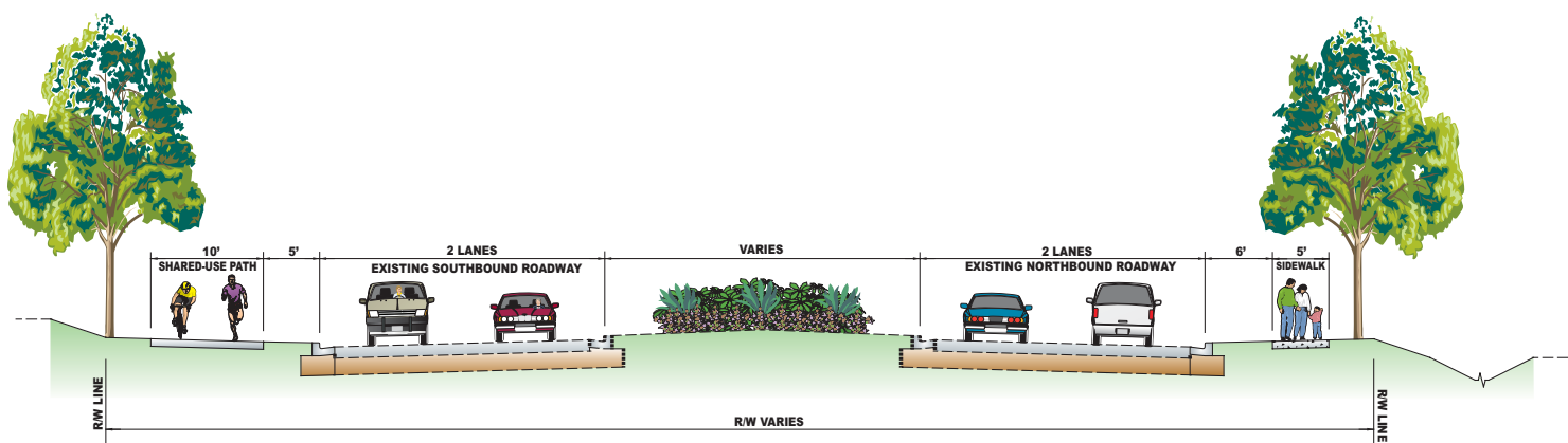
MIDCOUNTY HIGHWAY (MD 124) TYPICAL SECTION FROM GOSHEN ROAD TO MONTGOMERY VILLAGE AVE.
