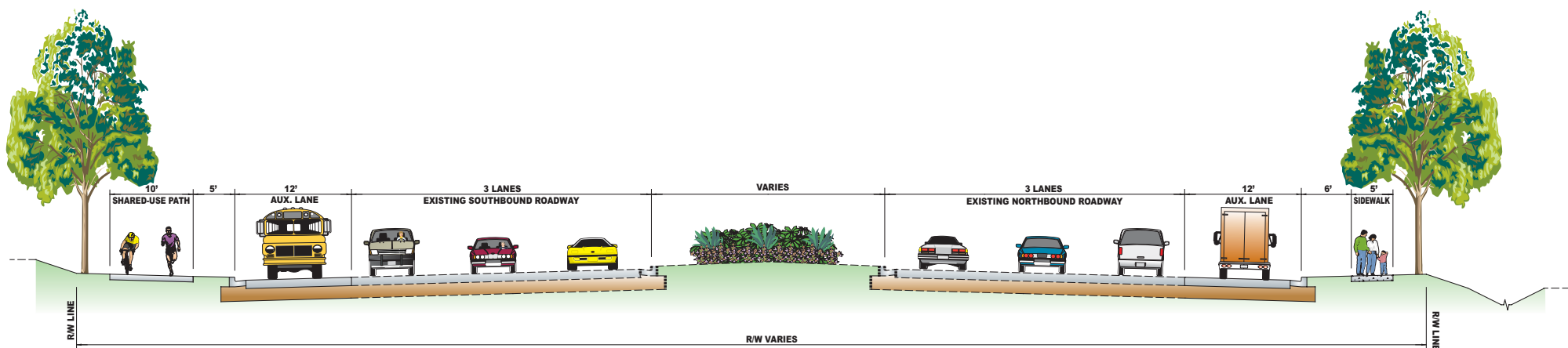
MD 355 TYPICAL SECTION FROM GUNNERS BRANCH ROAD TO MIDDLEBROOK ROAD FROM GERMANTOWN ROAD TO SHAKESPEARE BLVD.
