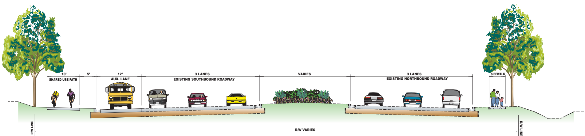
MD 355 TYPICAL SECTION FROM SHAKESPEARE BLVD. TO FATHER HURLEY BLVD. / RIDGE ROAD (MD 27)
