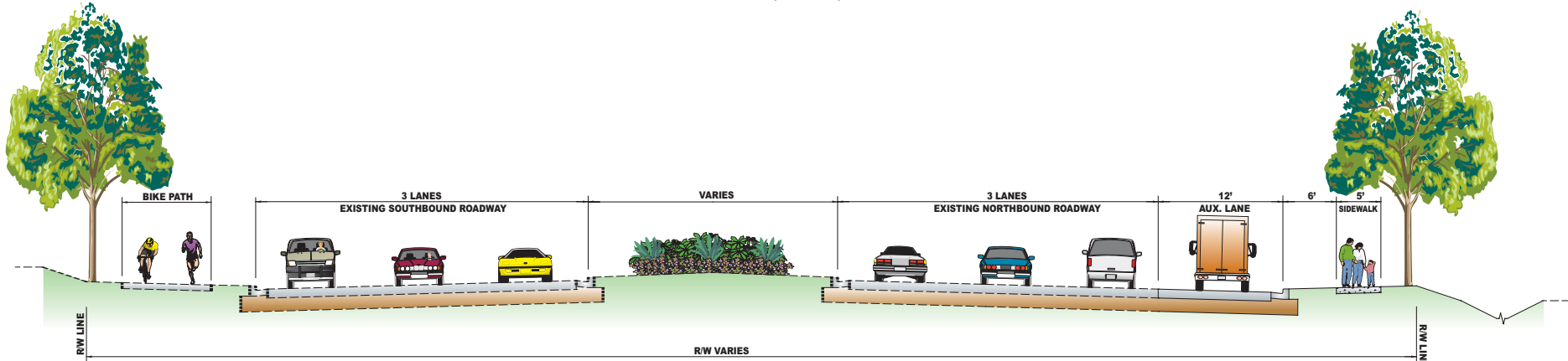
MD 355 TYPICAL SECTION FROM MONTGOMERY VILLAGE AVE. TO PROFESSIONAL DRIVE
