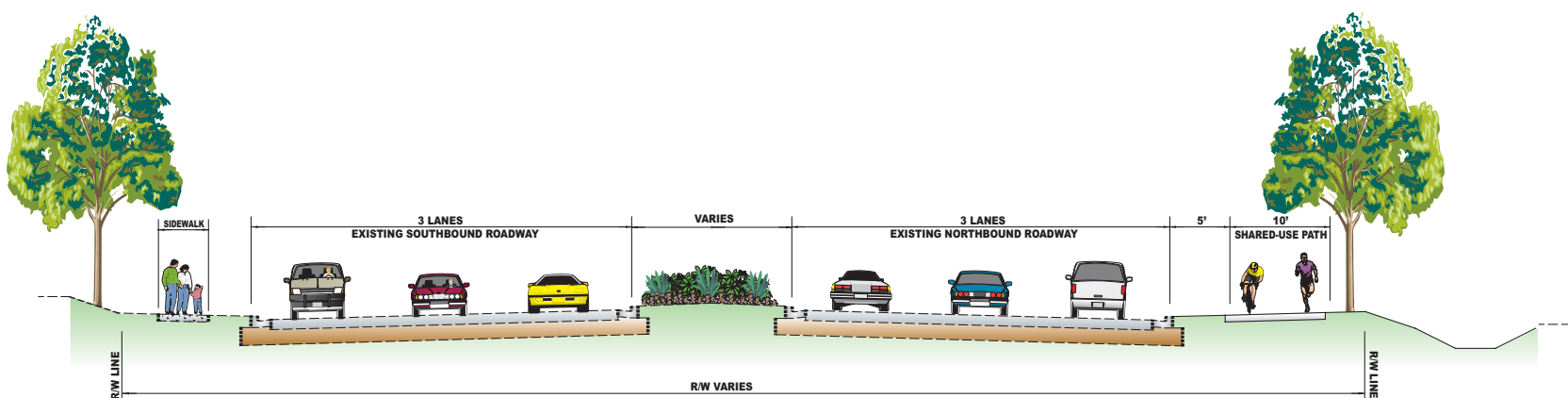
MONTGOMERY VILLAGE AVE. TYPICAL SECTION FROM MIDCOUNTY HIGHWAY (MD 124) TO MD 355
