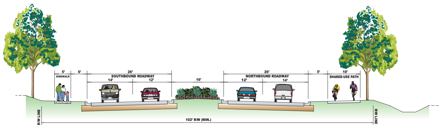
MIDCOUNTY HIGHWAY TYPICAL SECTION FROM MIDDLEBROOK ROAD TO RIDGE ROAD (MD 27)
