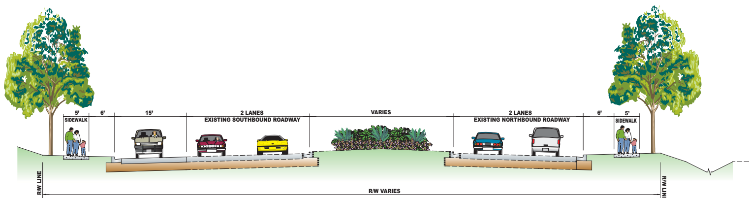
MIDCOUNTY HIGHWAY (MD 124) TYPICAL SECTION FROM GOSHEN ROAD TO MONTGOMERY VILLAGE AVE.
