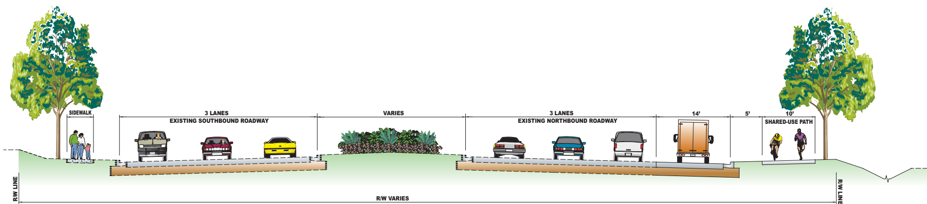
MONTGOMERY VILLAGE AVE. TYPICAL SECTION FROM MIDCOUNTY HIGHWAY (MD 124) TO MD 355
