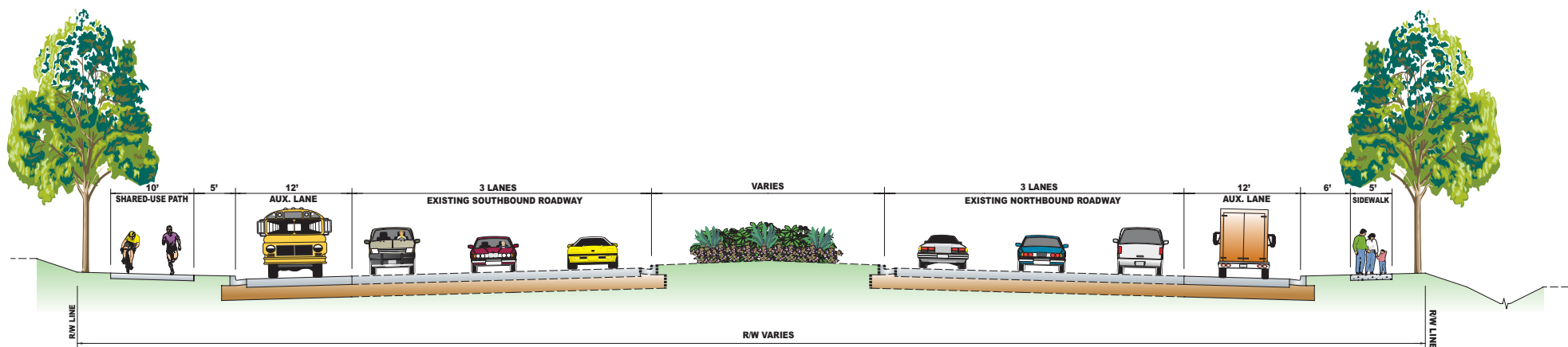
MD 355 TYPICAL SECTION FROM MONTGOMERY VILLAGE AVE. TO PROFESSIONAL DRIVE FROM GUNNERS BRANCH ROAD TO MIDDLEBROOK ROAD
