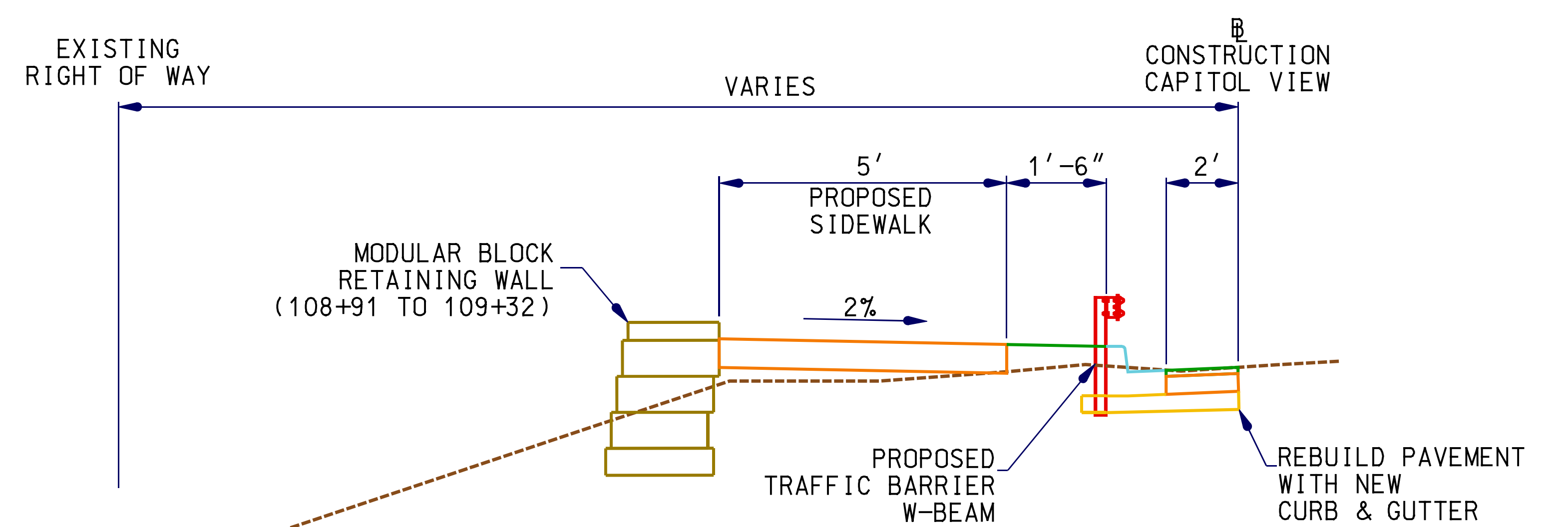
CAPITOL VIEW AVENUE – TYPICAL SECTION WITH BLOCK WALL
