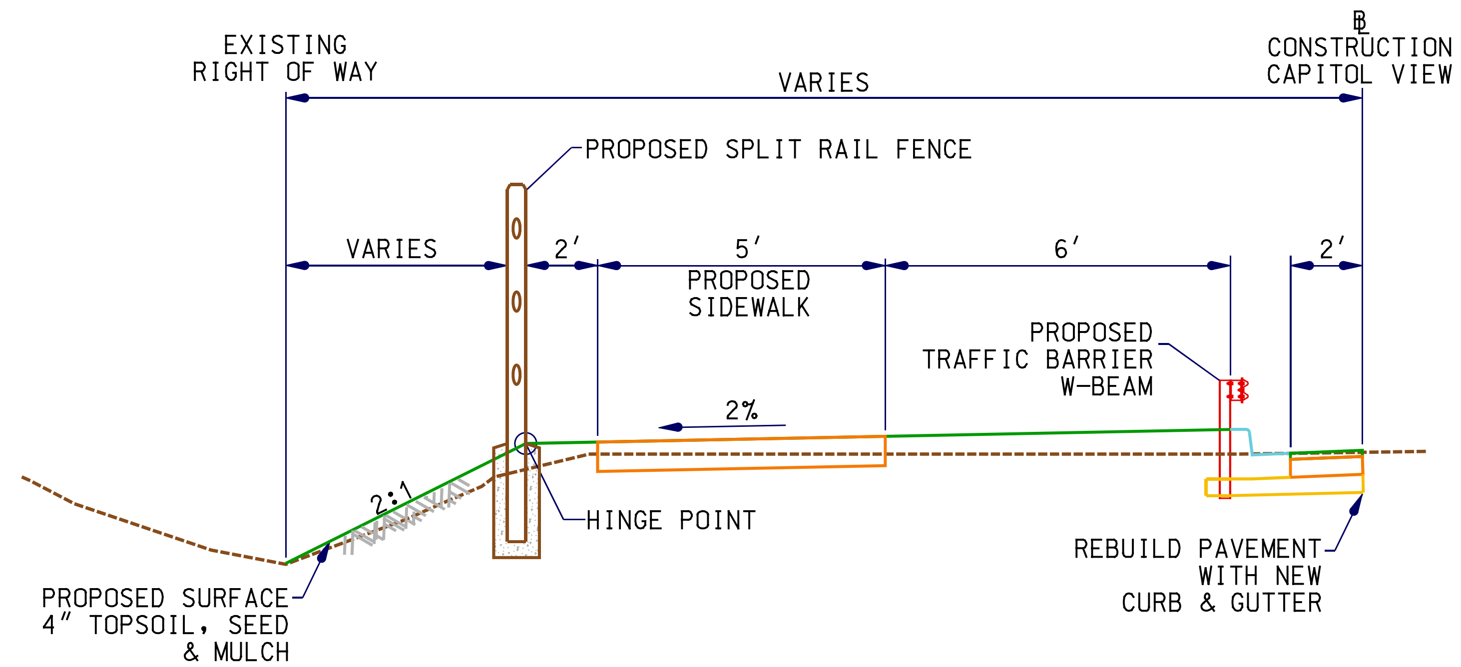
CAPITOL VIEW AVENUE – FILL SECTION
