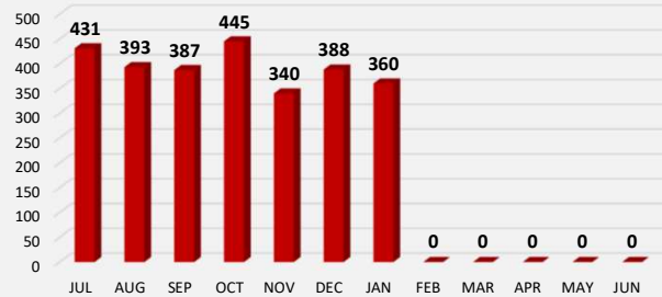
FY21- Criminal
