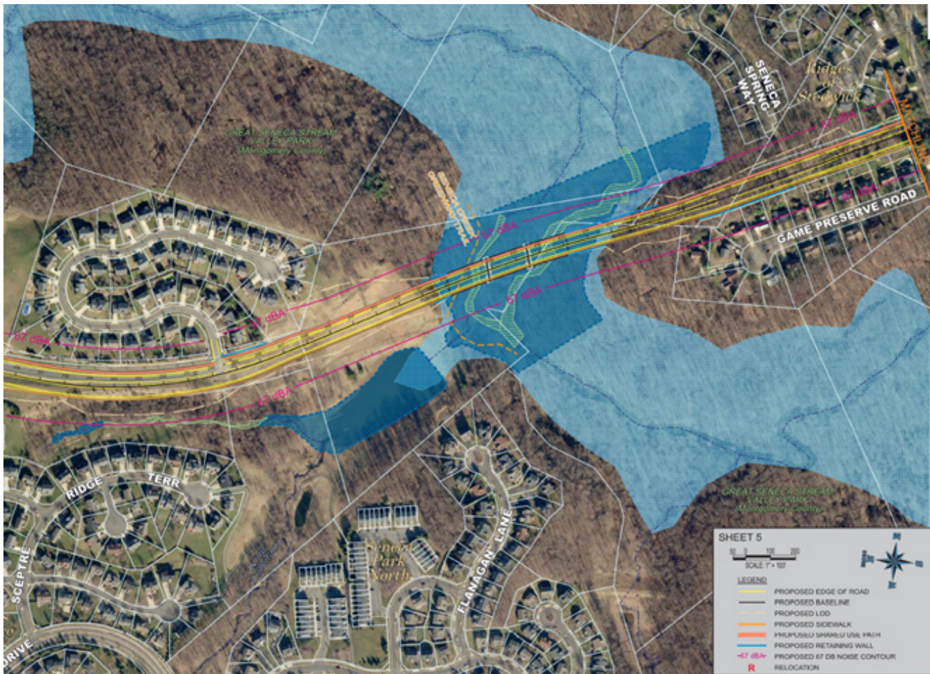
Figure 11. Proposed M83 500-foot bridge crossing of Seneca Creek.
