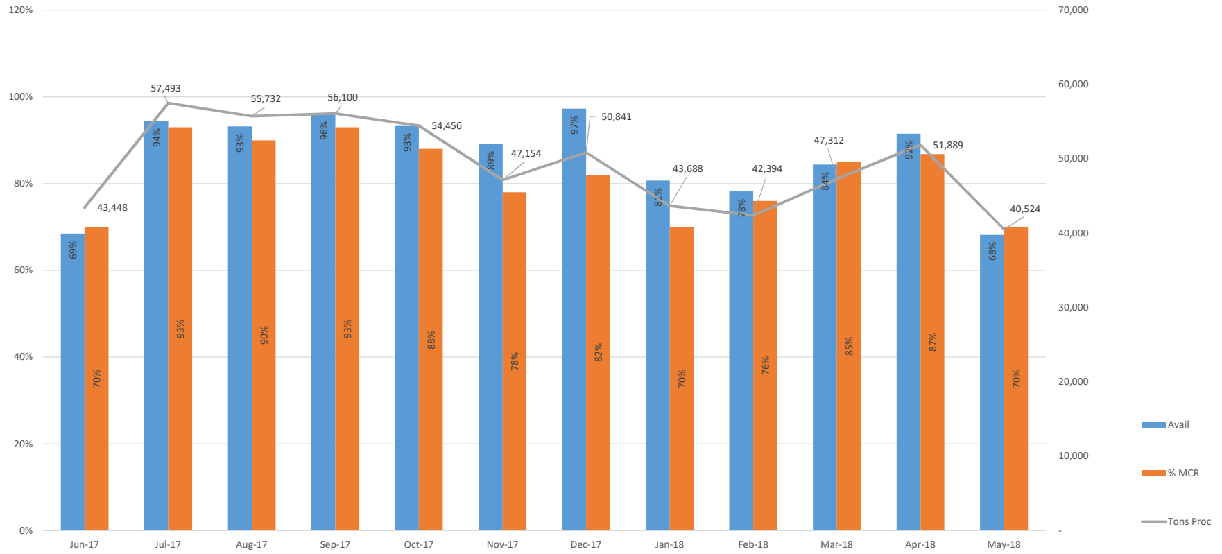
12 Month Rolling - Availability - Percent MCR - Tons Processed
