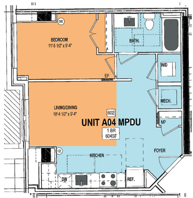
Floor Plan
