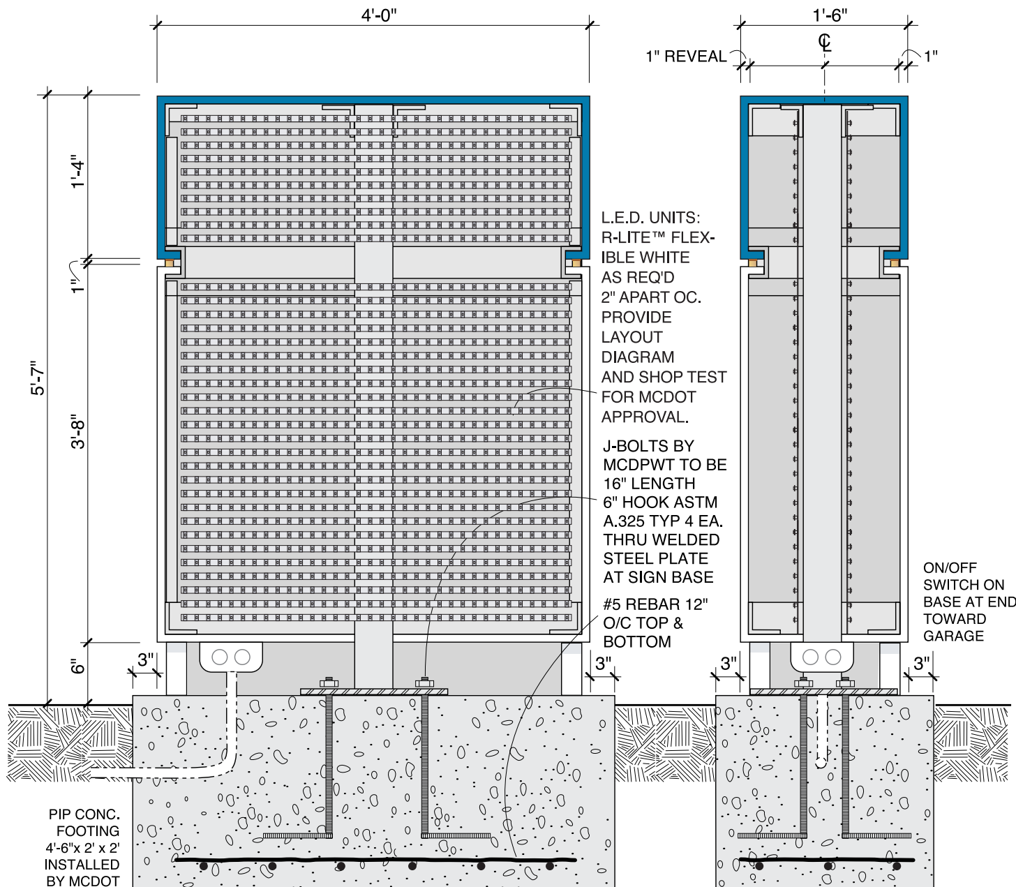
ID4 - THE COUNTY PYLON SIGN - FRONT & SIDE VIEWS
