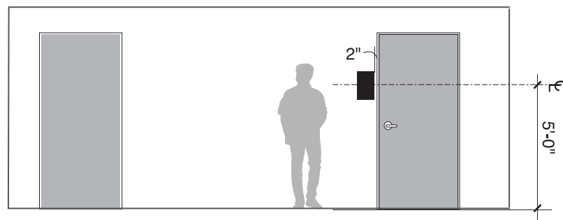
CO3 - RESTROOM PLAQUE - SIGN LOCATION
