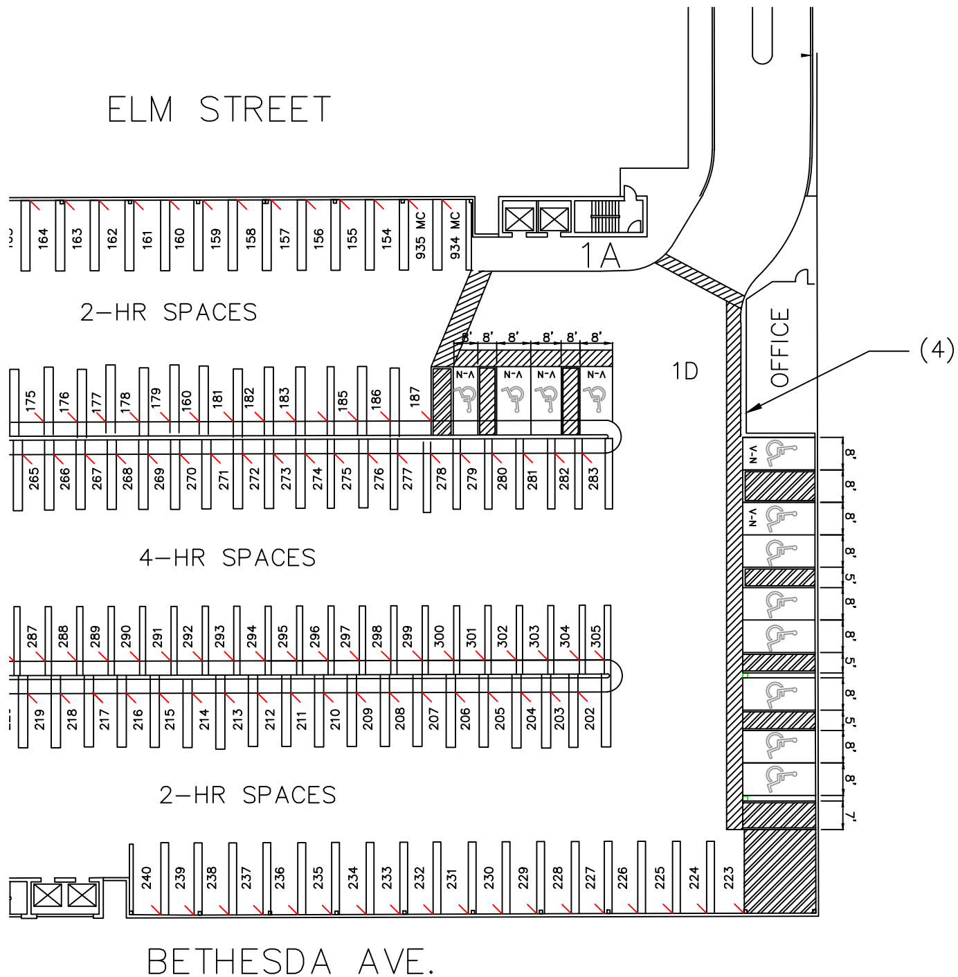
GARAGE 57 FIRST LEVEL PLAN
