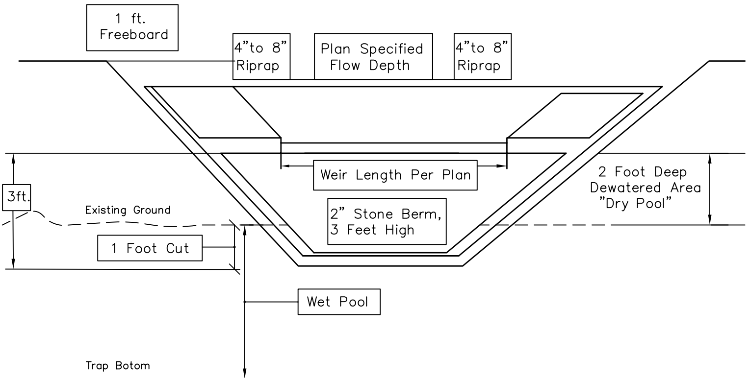
SECTION BB NO SCALE
