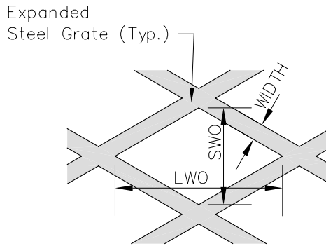
Expanded Steel Grate Opening Detail Not To Scale
