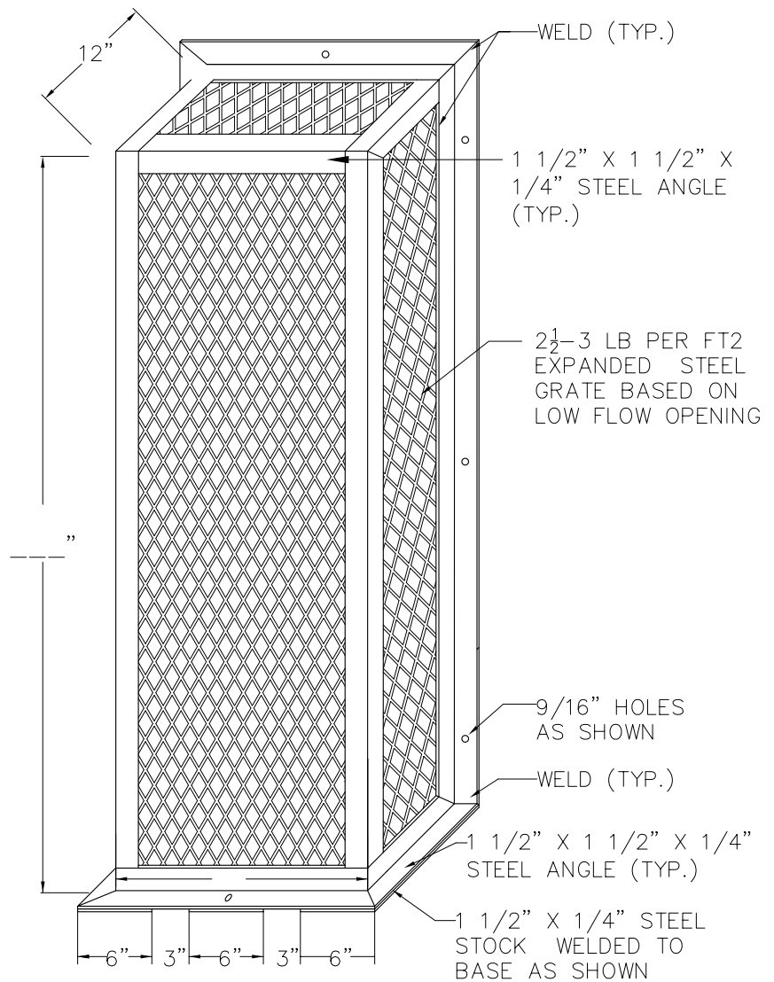
Expanded Steel Grate Opening Detail Not To Scale
