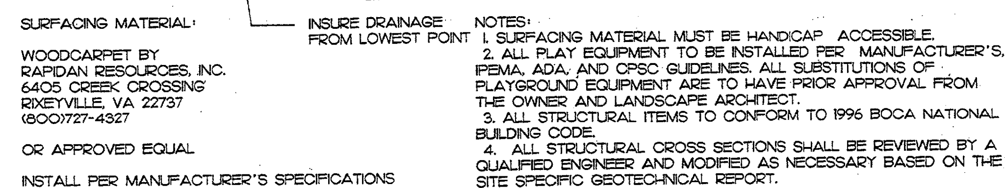
8 TOT LOT SURFACING IOE-27 L-II PICTORIAL NTS
