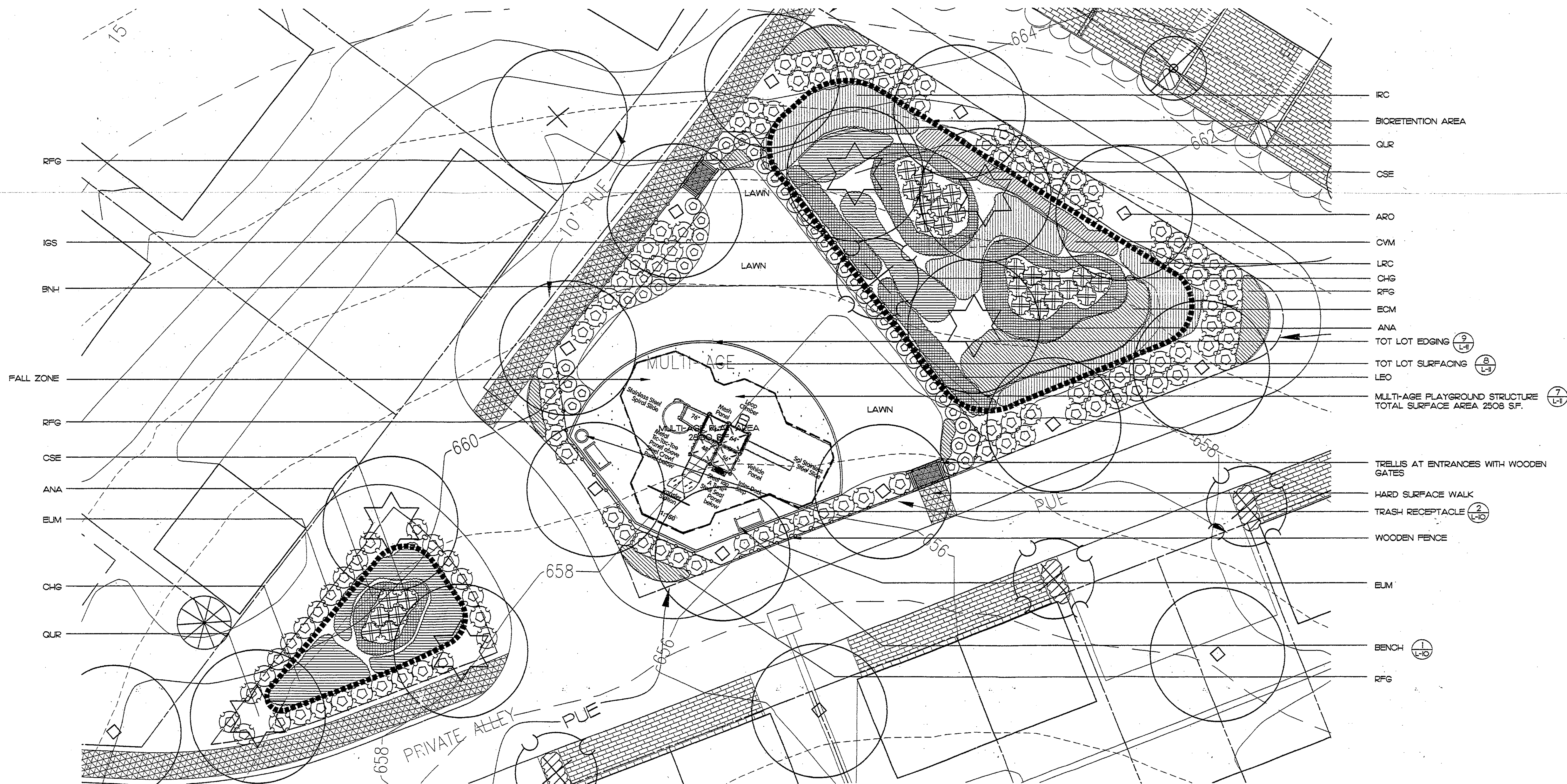
1 MULTI-AGE PLAY AREA ENLARGEMENT L-6 PLAN 1" = 10'
