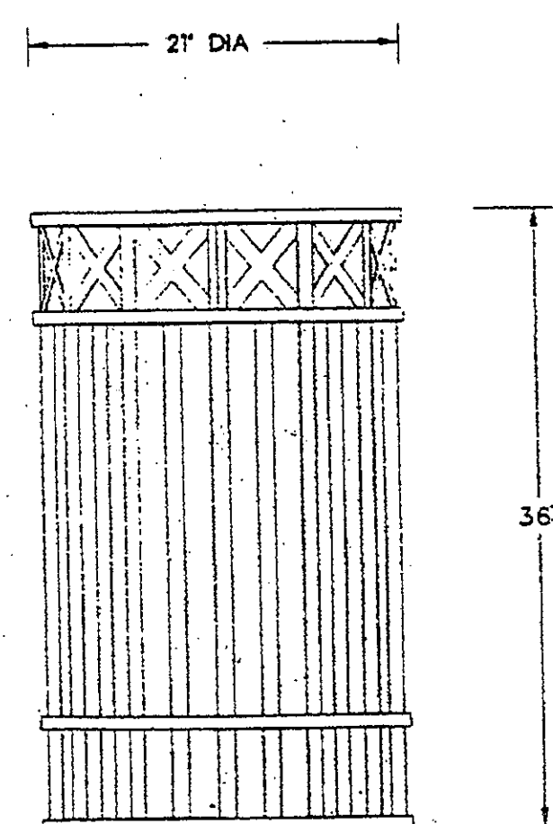
2 TRASH RECEPTACLE L-10 PICTORIAL
