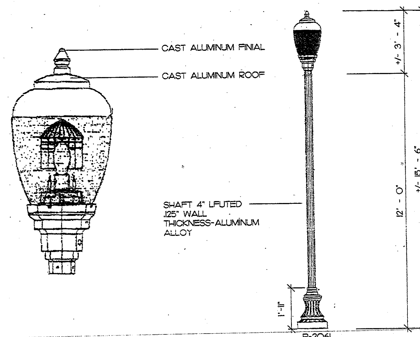
6 PARKING AREA LUMINAIRE L-10 PICTORIAL
