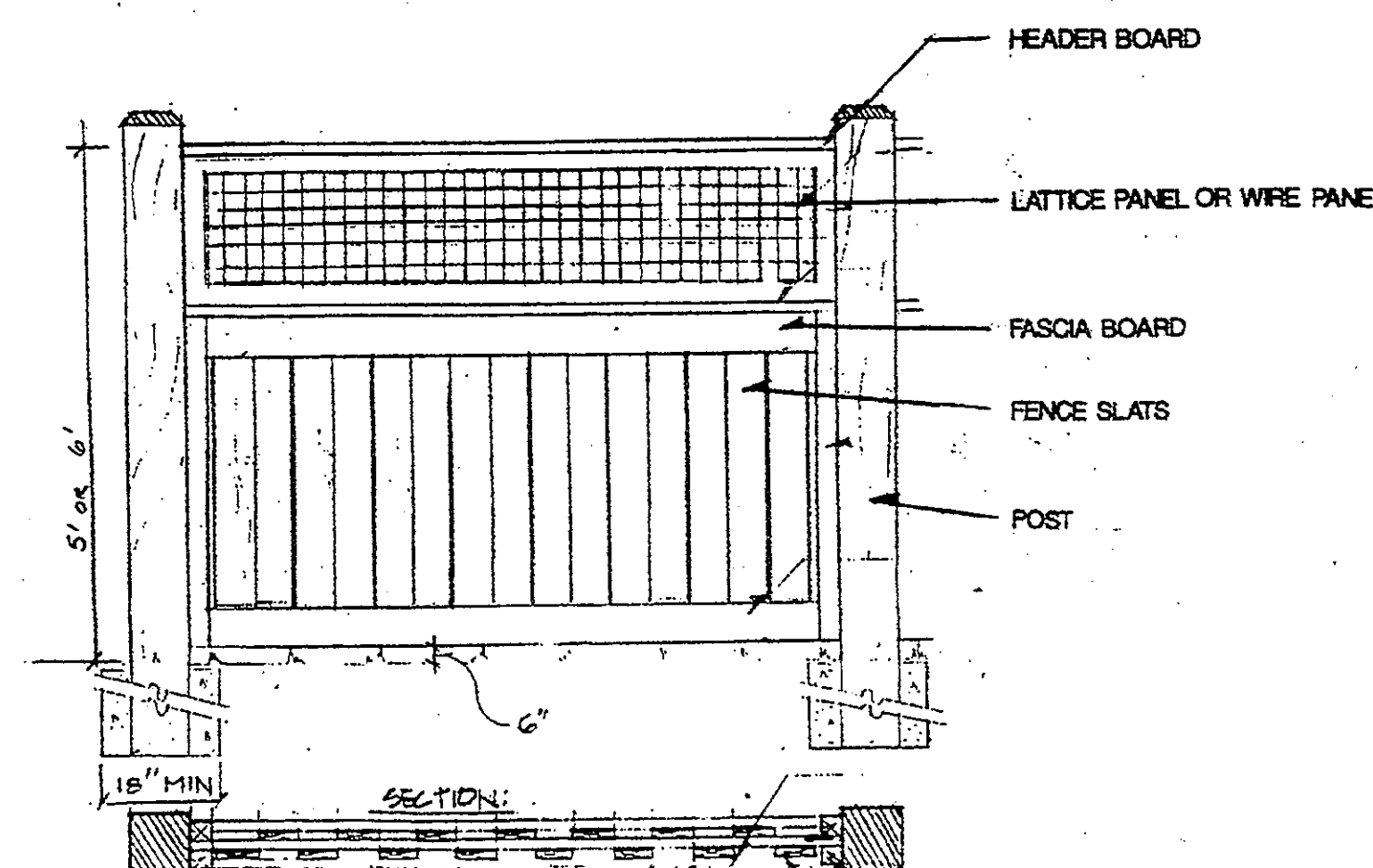
8 WOOD FENCE L-10 ELEVATION
