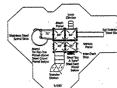
7 MULTI-AGE PLAYGROUND STRUCTURE IOE-059 L-II PICTORIAL NOT TO SCALE
