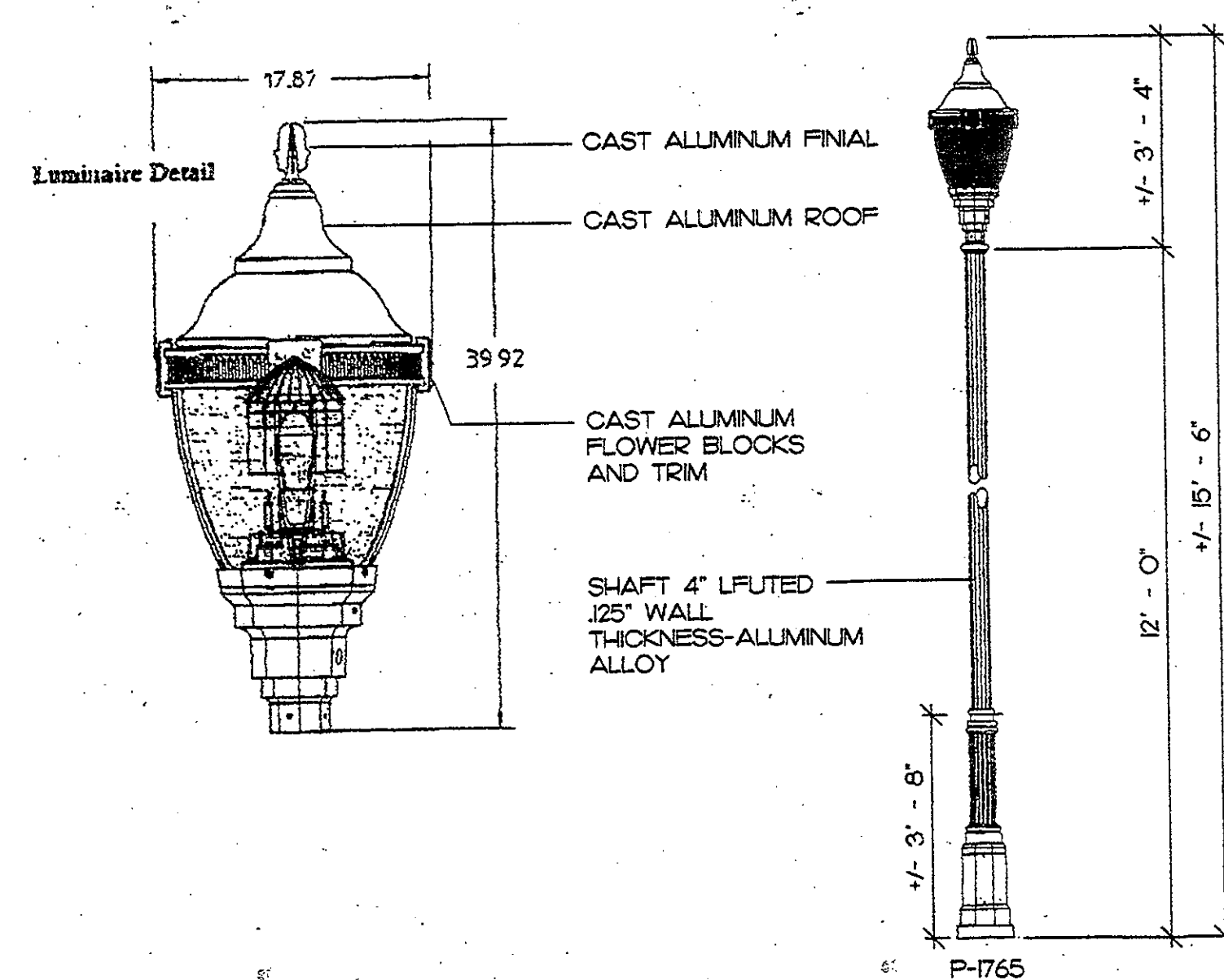
5 STREETLIGHT LUMINAIRE L-10 PICTORIAL
