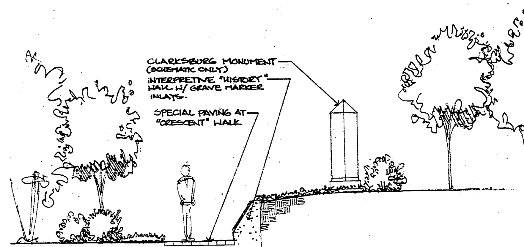
9 CLARKE MEMORIAL WALL/MONUMENT L-10 SECTION
