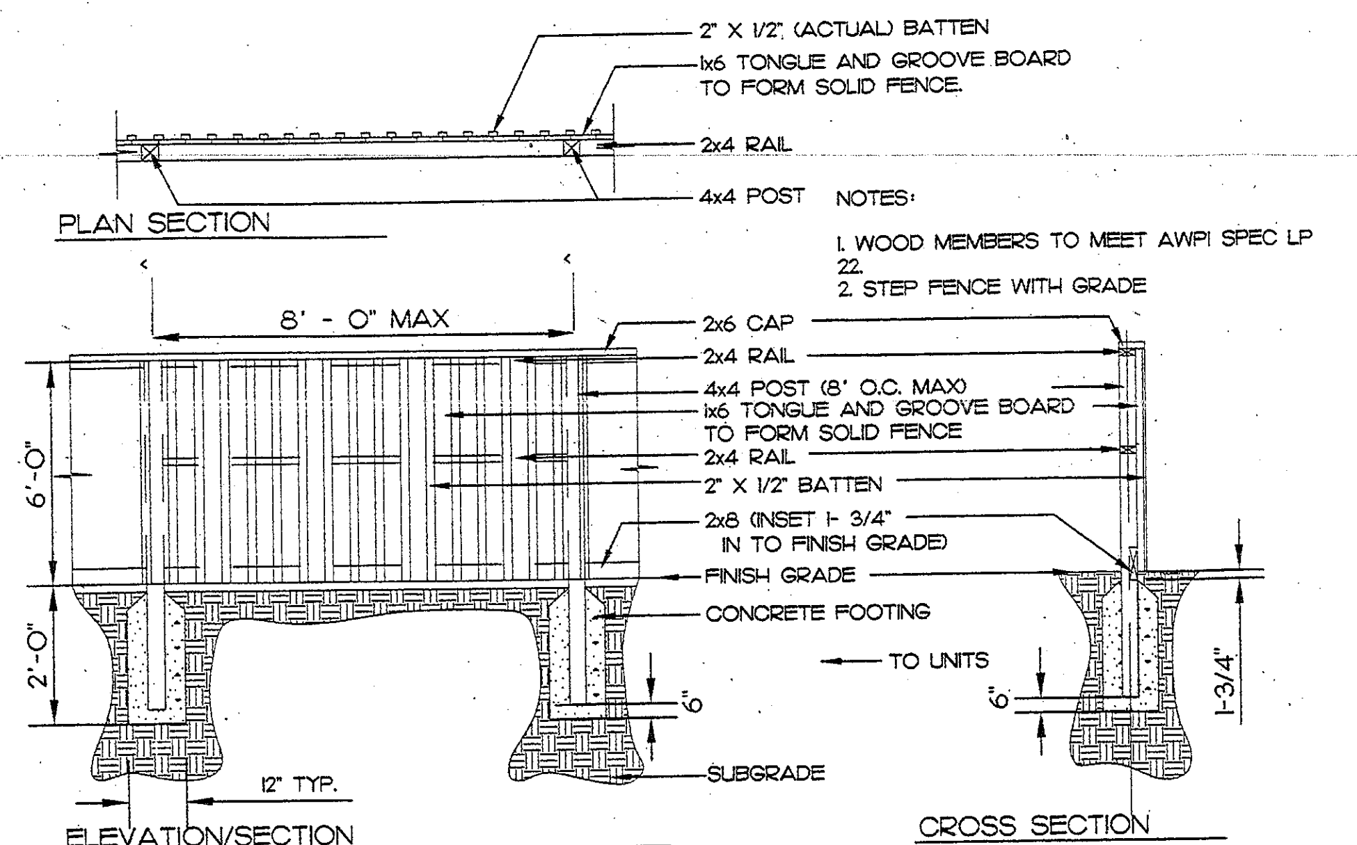
4 NOISE ABATEMENT SCREEN L-10 PLAN/SECTION/ELEVATION
