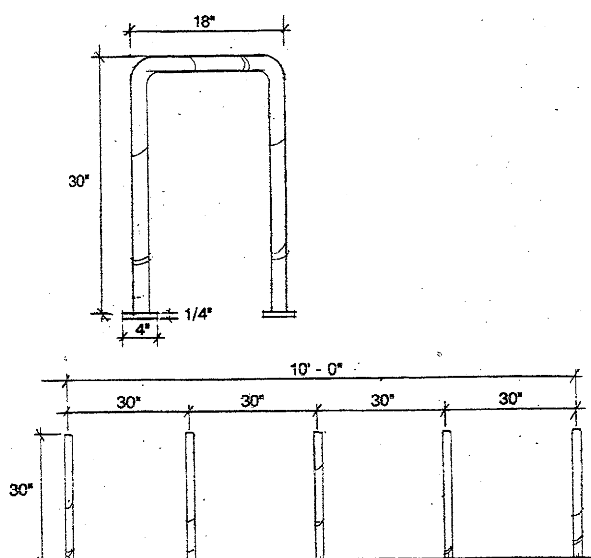
3 BIKE RACK L-10 PICTORIAL
