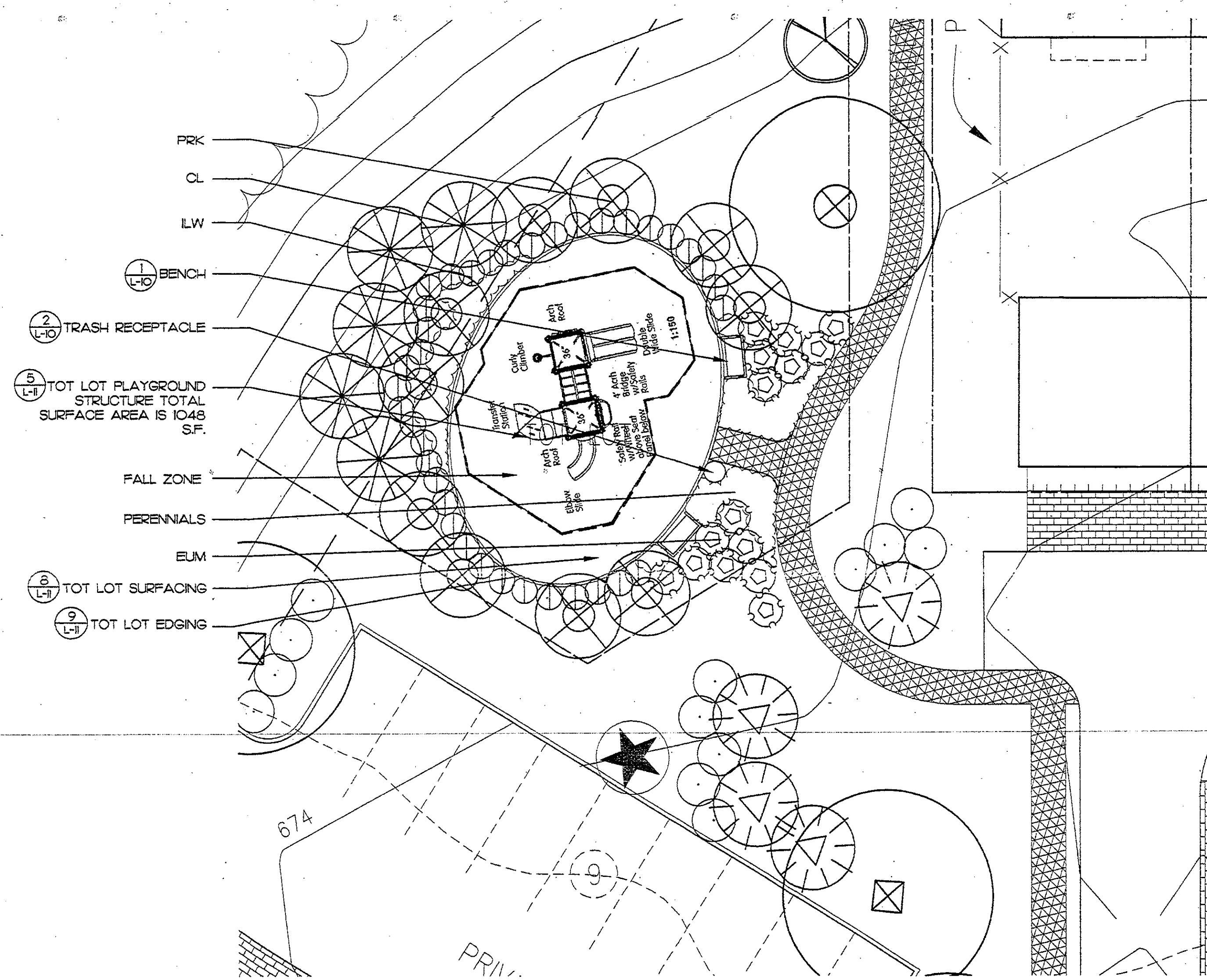
2 TOT LOT A ENLARGEMENT L-6 PLAN 1" = 10'
