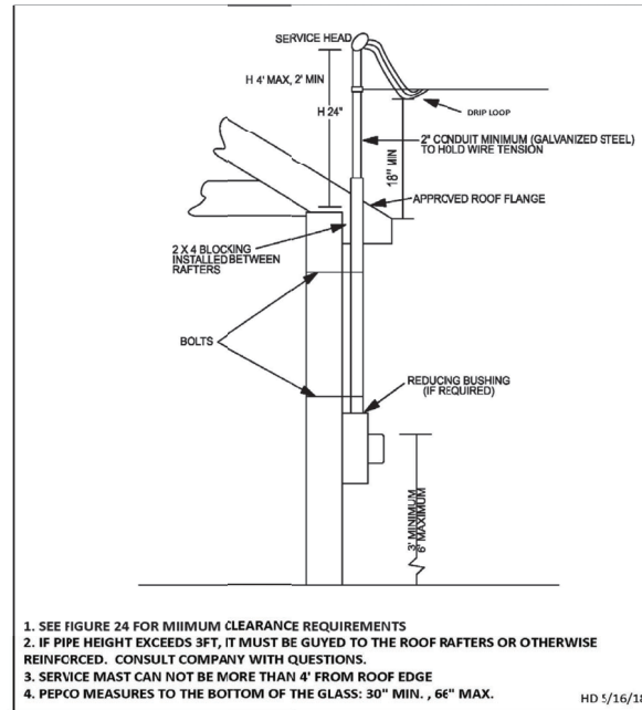
SERVICE MAST ~FIGURE #25~
