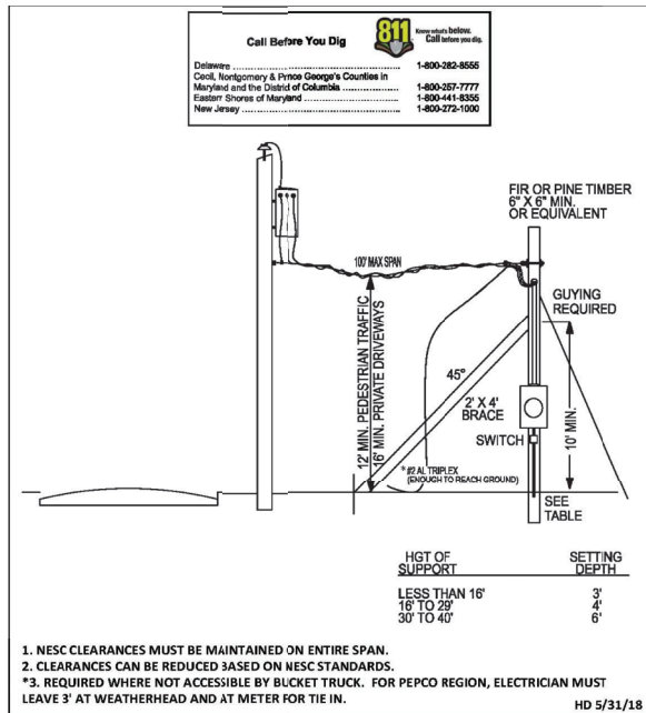
OVERHEAD TEMPORARY SERVICE (ACROSS PRIVATE DRIVE) ~FIGURE #22~
