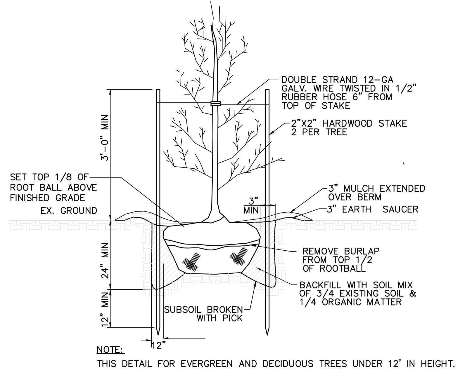
PLANTING DETAIL NOT TO SCALE
