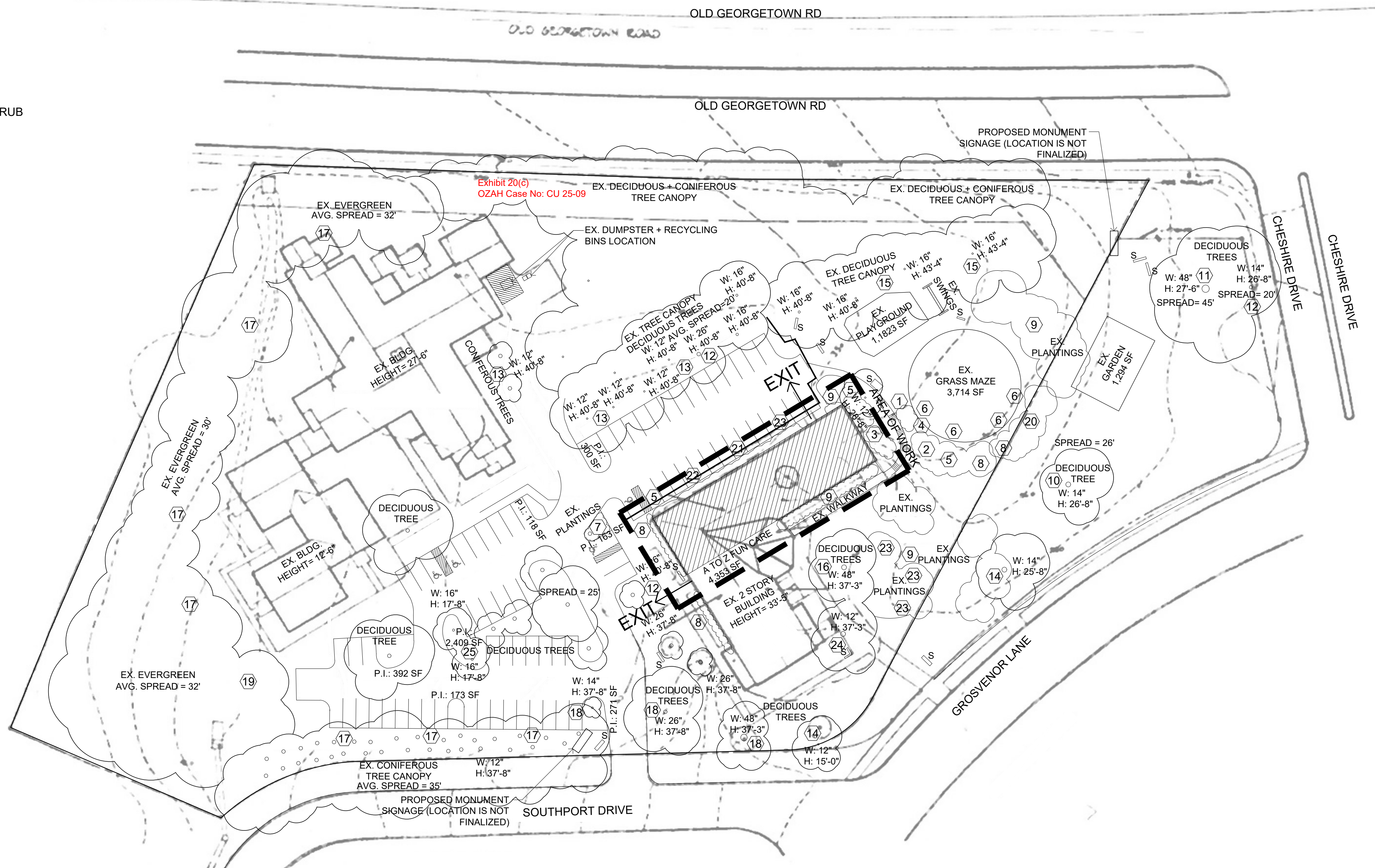
1 LANDSCAPING PLAN
