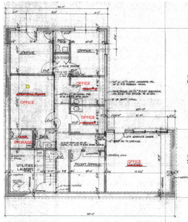
Basement Floorplan (1,920 SF)
