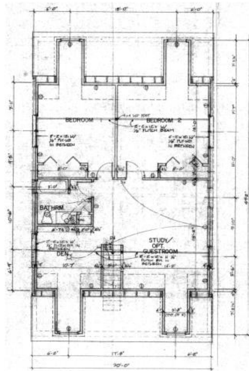
Second Floorplan (1,165 SF)
