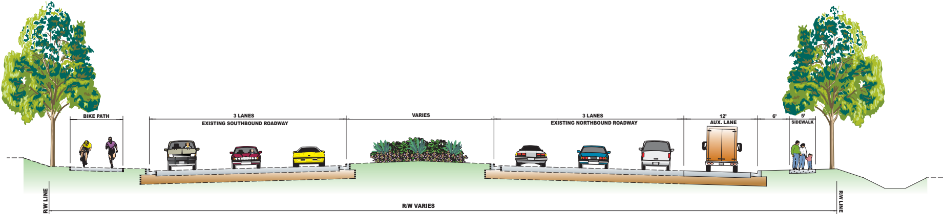
MD 355 TYPICAL SECTION FROM CHRISTOPHER AVE. TO WATKINS MILL ROAD
