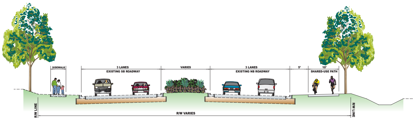
MONTGOMERY VILLAGE AVE. TYPICAL SECTION FROM MIDCOUNTY HIGHWAY (MD 124) TO MD 355
