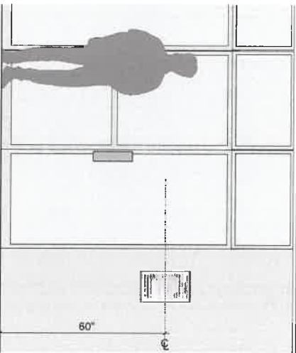
IN403 - DISPLAY WINDOW UNITS - ELEVATION AT LOCATION Scale: 3/8" = 1'-0"
