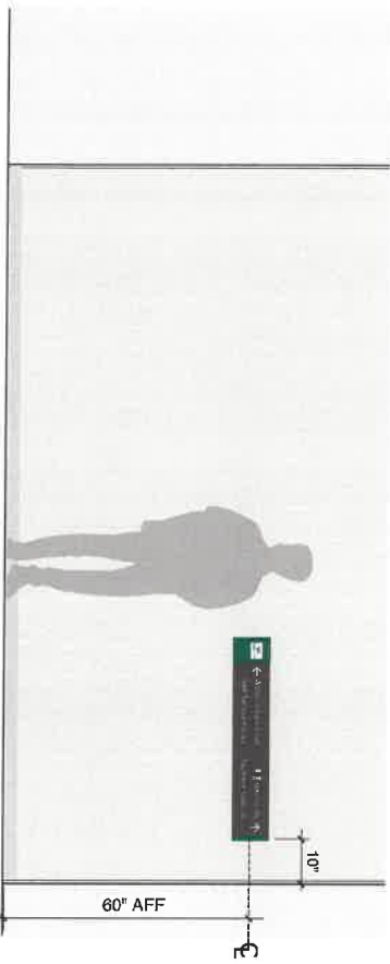
DR501 DIRECTIONAL INFO - EXAMPLE LOCATION 7th Floor 08 Scale: 3/8"=1'-0"
