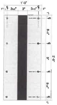
PLAN VIEW
