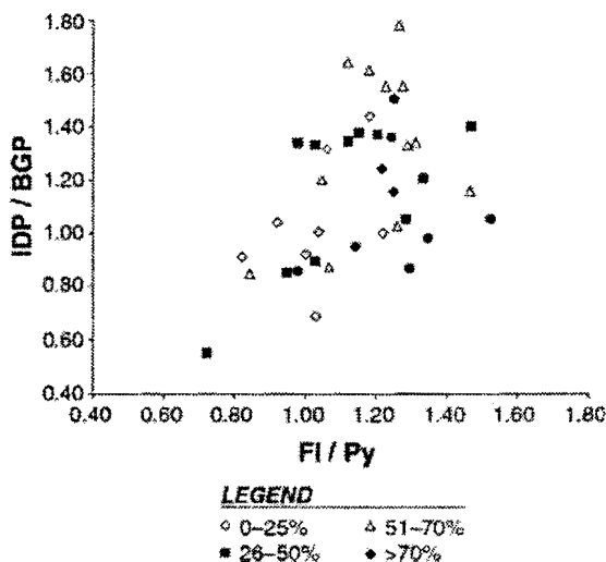
Figure 5. Comparison of double-ratio plot results to chemical mass balance (CMB) model output.
