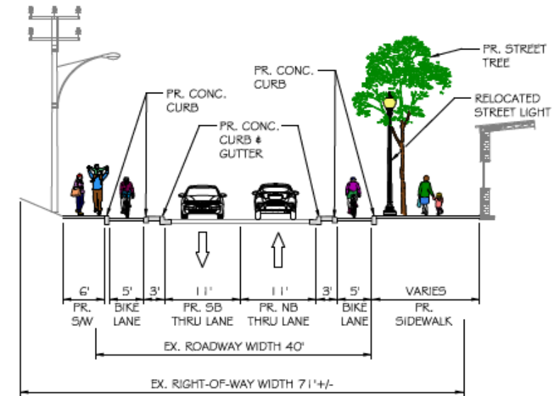
Figure 37- Proposed Typical Section, Flower Avenue from the Flower Avenue Urban Park to Arliss Street (MD 594-D)
