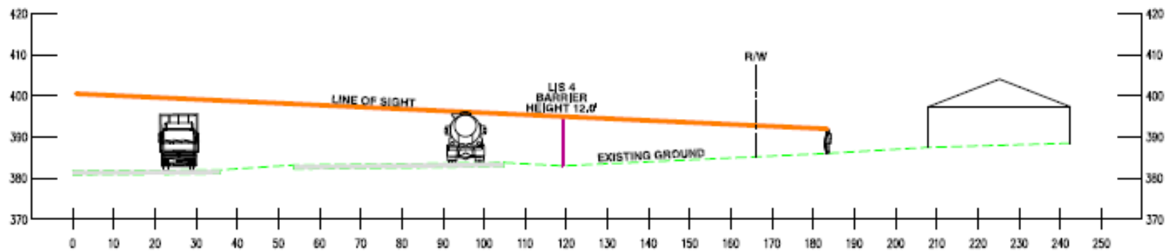
SECTION E-E
