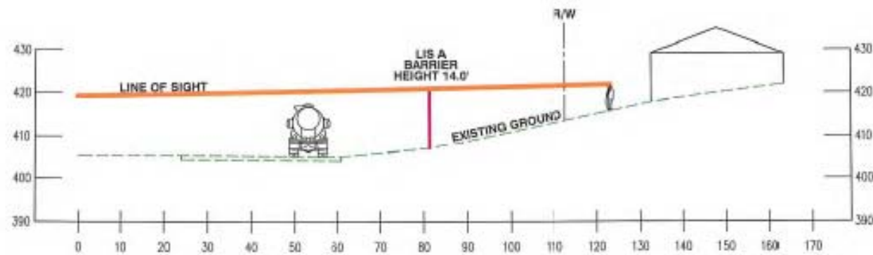
SECTION C-C
