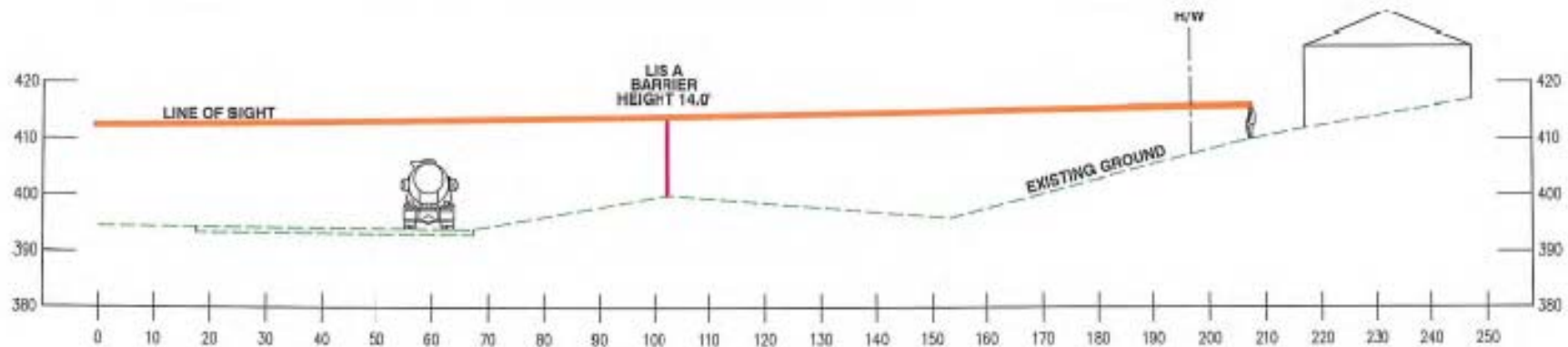
SECTION B-B
