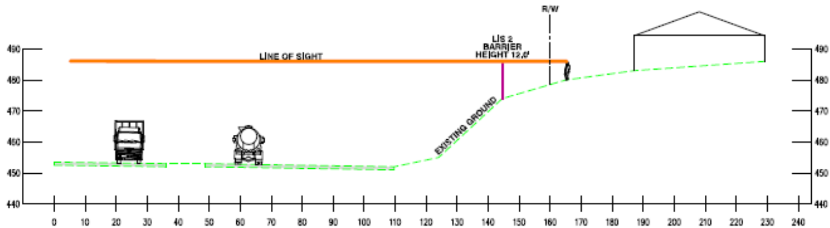
SECTION B-B
