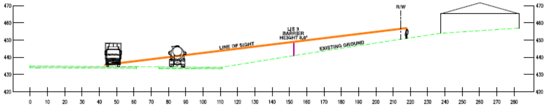
SECTION C-C
