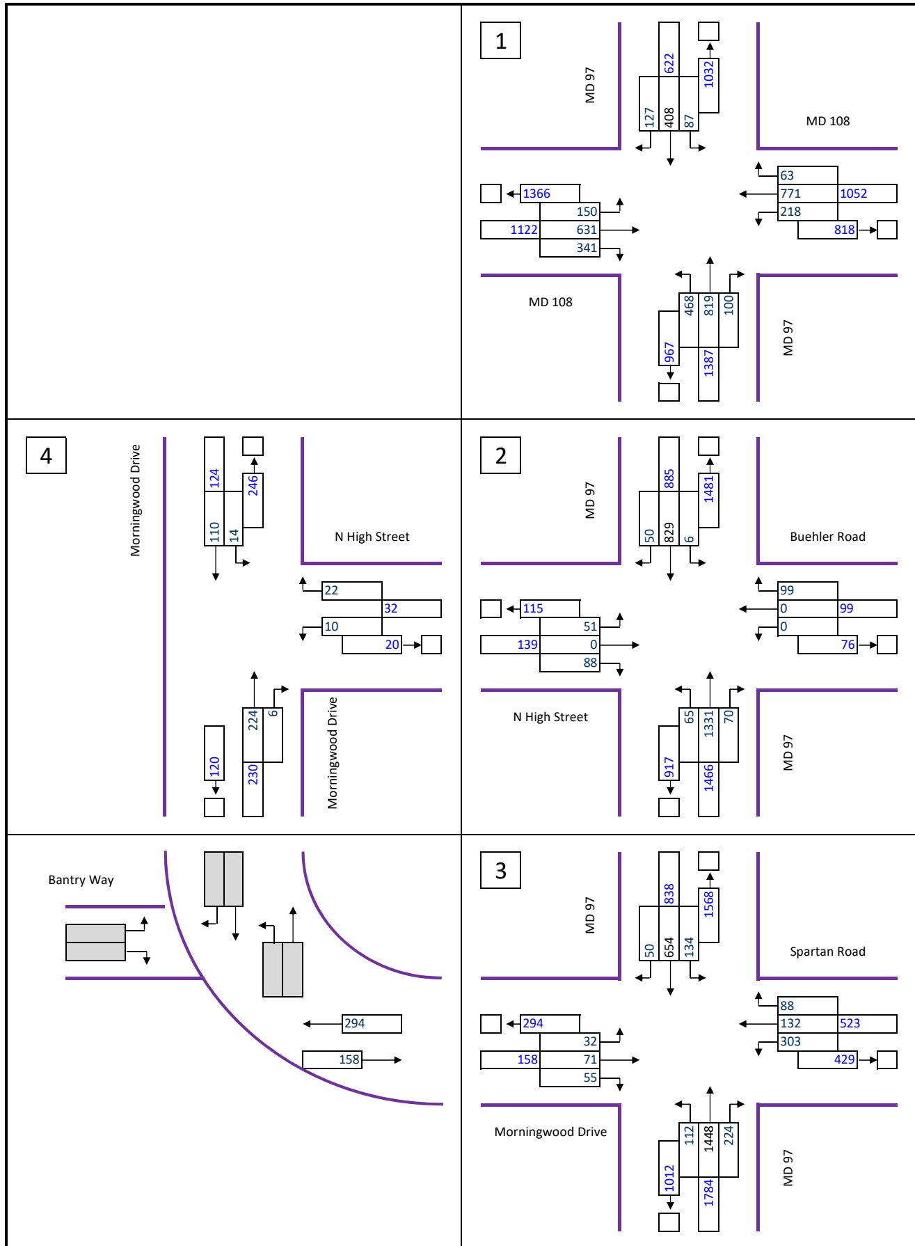
D10: AM Peak Hour Traffic Volumes with North High Street Connection
