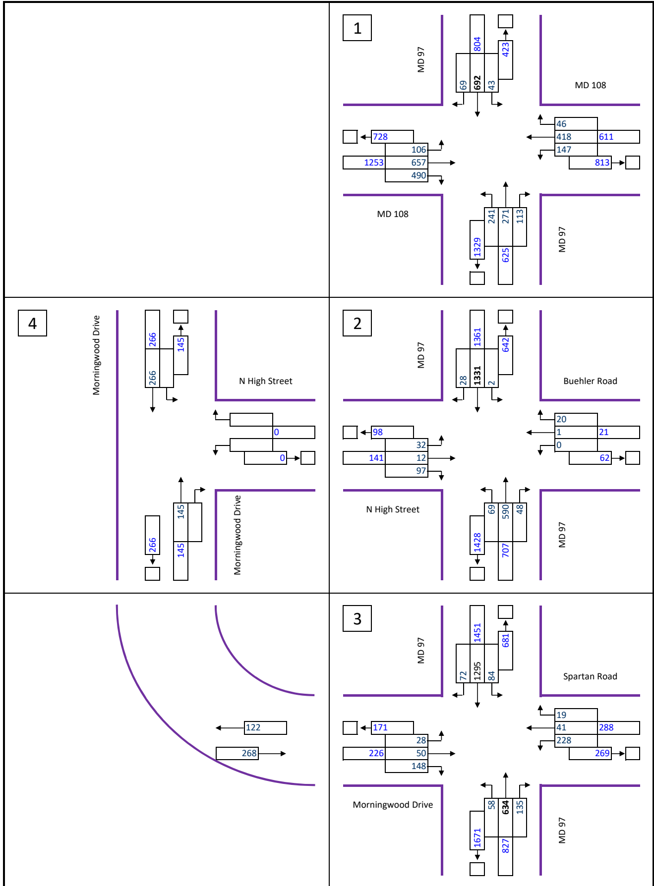
D-3: Existing Peak Hour Traffic Volumes - AM Adjusted
