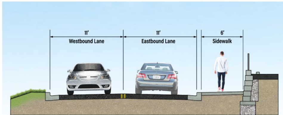
PROPOSED NORTH HIGH STREET - A2-A2
