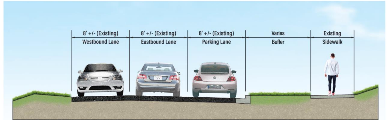
EXISTING NORTH HIGH STREET WITH PARKING - B-B
