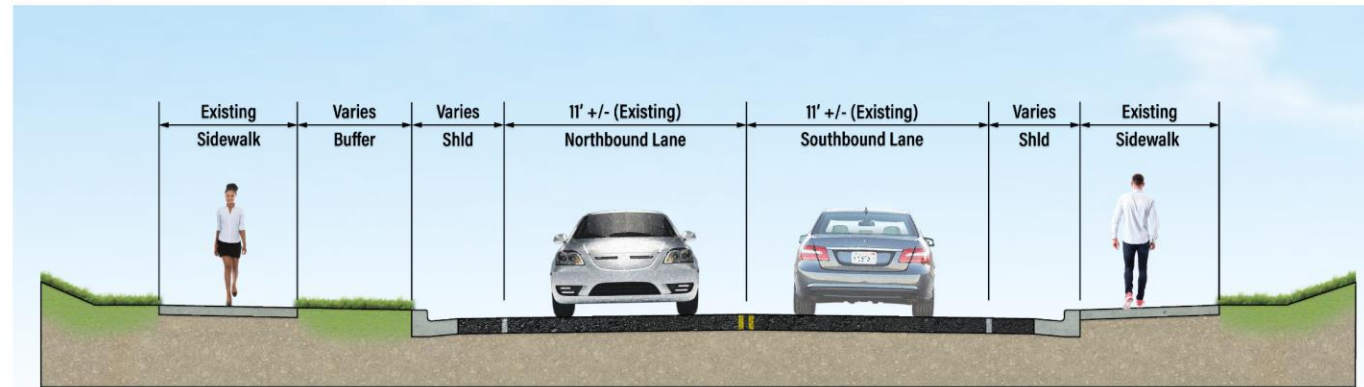
EXISTING MORNINGWOOD DRIVE - C-C
