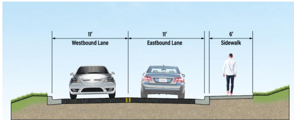
PROPOSED NORTH HIGH STREET - A1-A1
