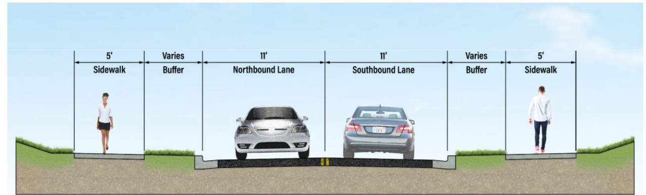
PROPOSED MORNINGWOOD DRIVE - C-C
