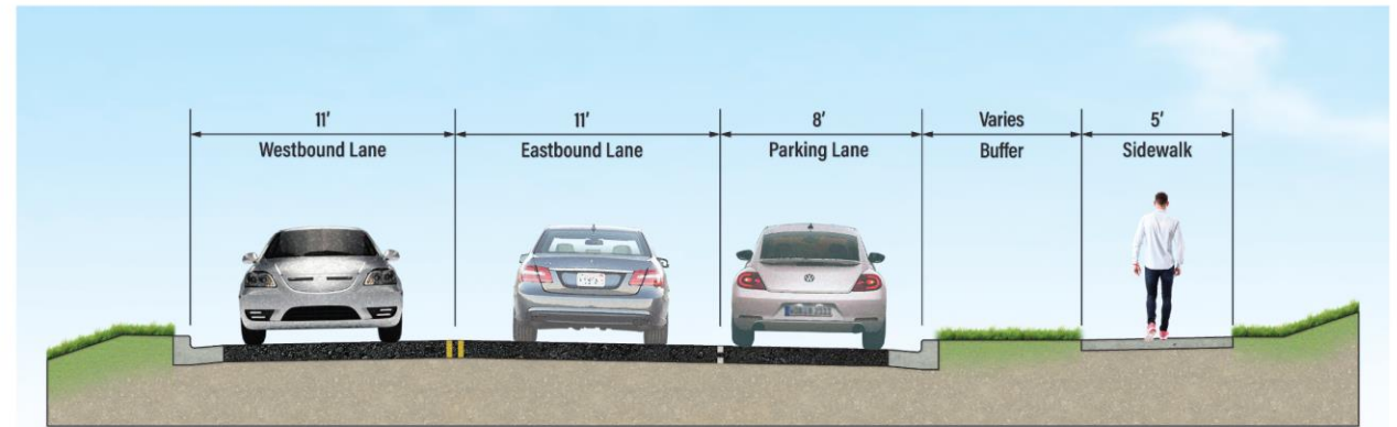
PROPOSED NORTH HIGH STREET WITH PARKING - B-B
