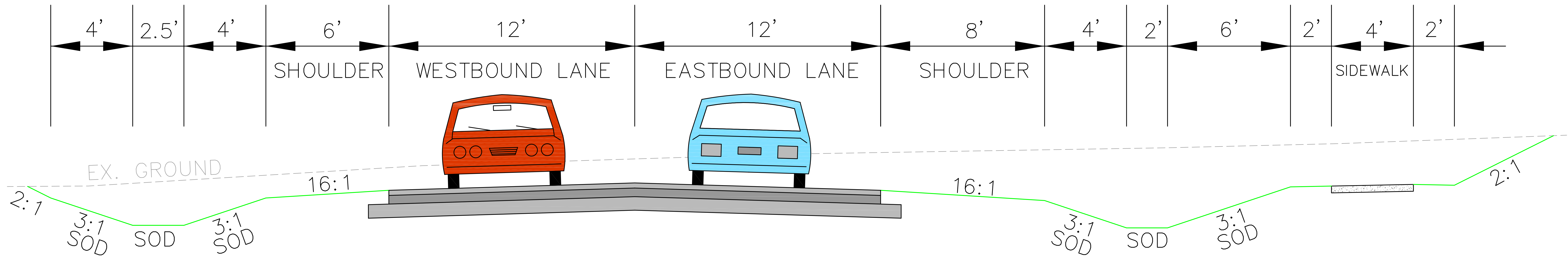
PROPOSED RAINBOW DRIVE STA. 15+09.12 TO 17+01.75
