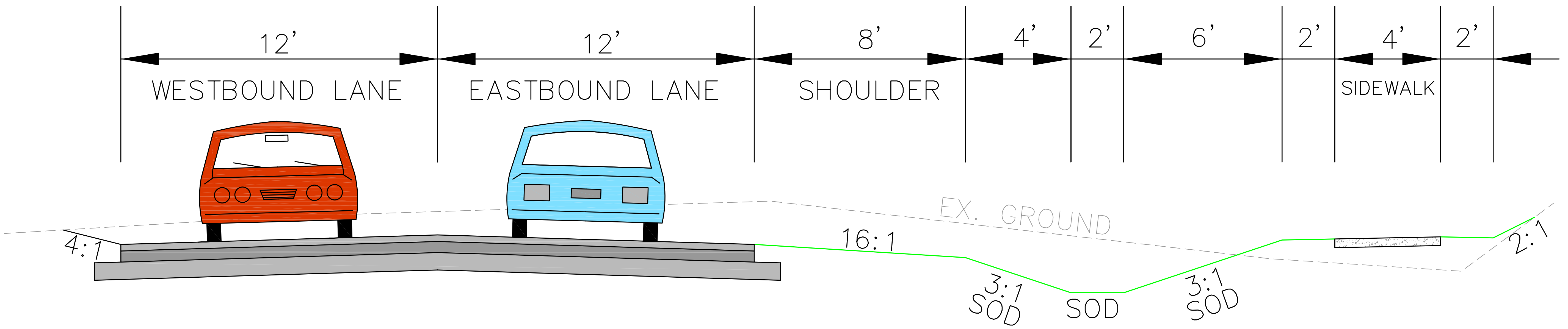
PROPOSED RAINBOW DRIVE STA. 17+01.75 TO 17+47.65
