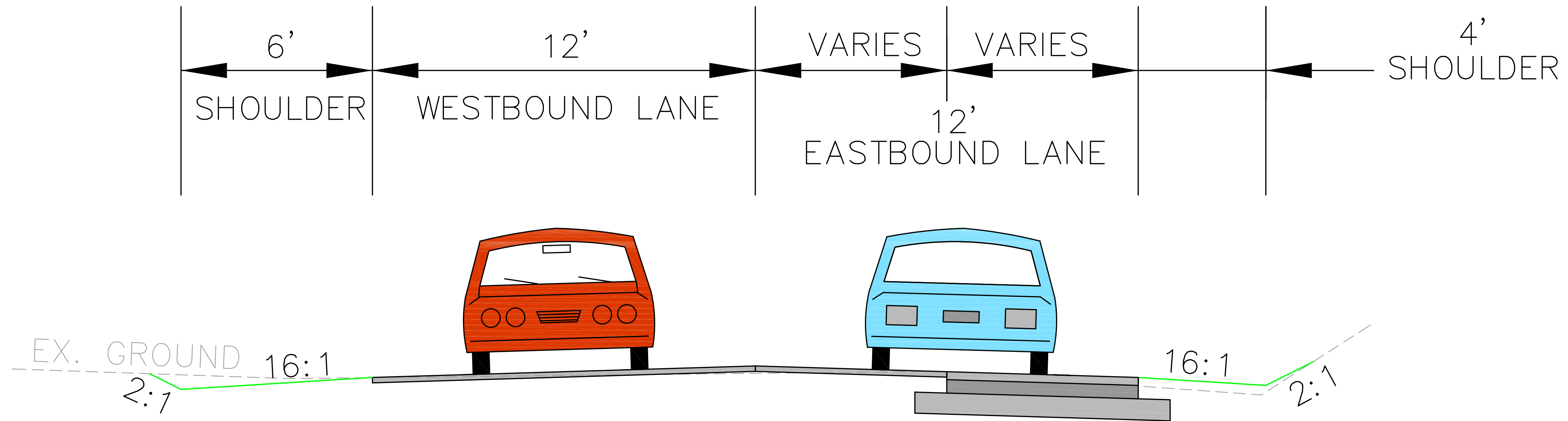
PROPOSED RAINBOW DRIVE STA. 17+47.65 TO 18+73
