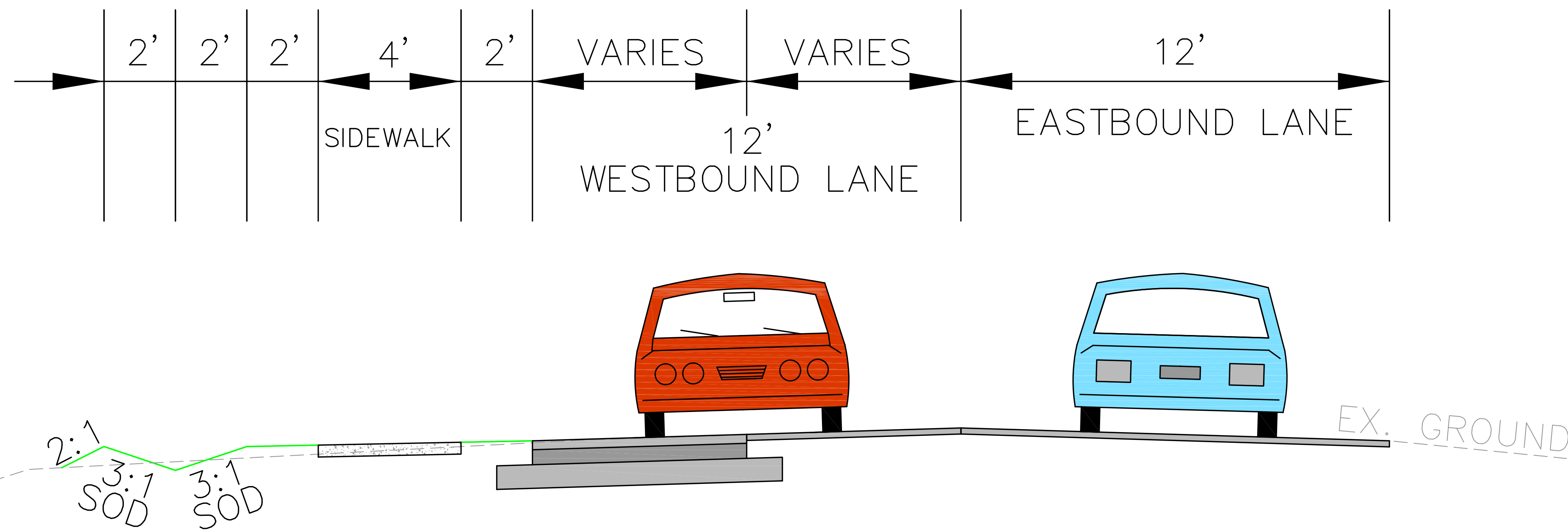
PROPOSED THOMPSON ROAD
