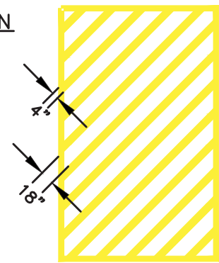
YELLOW, 4" WIDTH, 18" SPACING, 45 DEGREE ANGLE FIRE LANE STRIPING DETAIL N.T.S.
