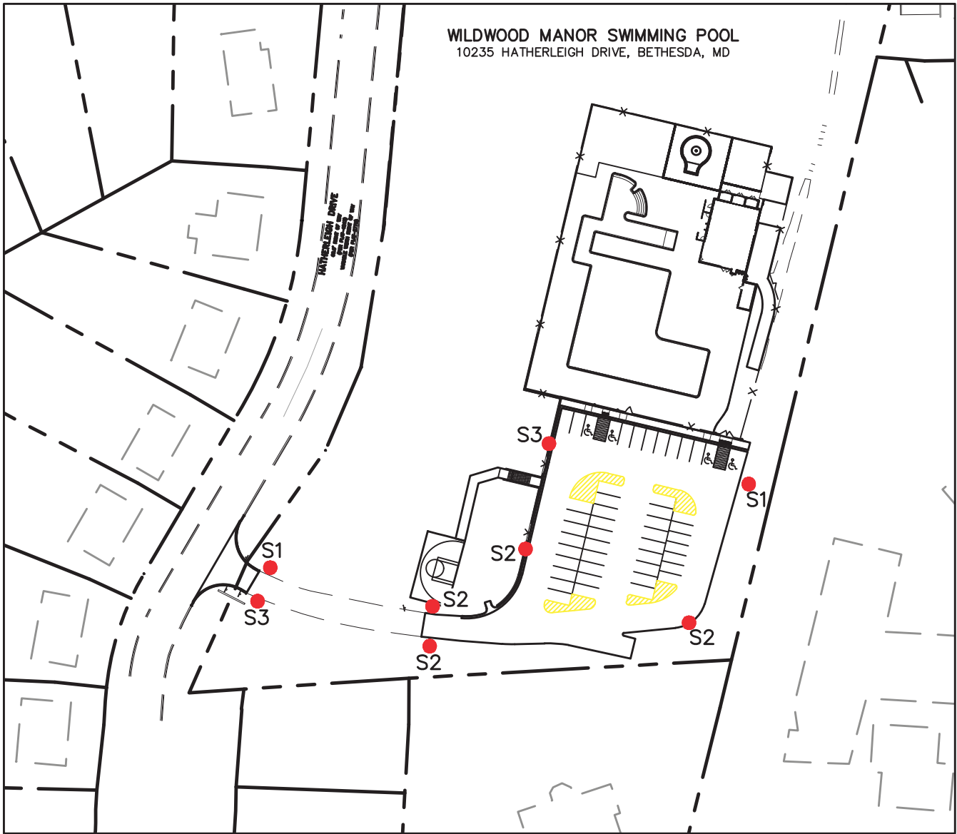
FIRE LANE SIGNAGE AND STRIPING PLAN SCALE: 1" = 100'
