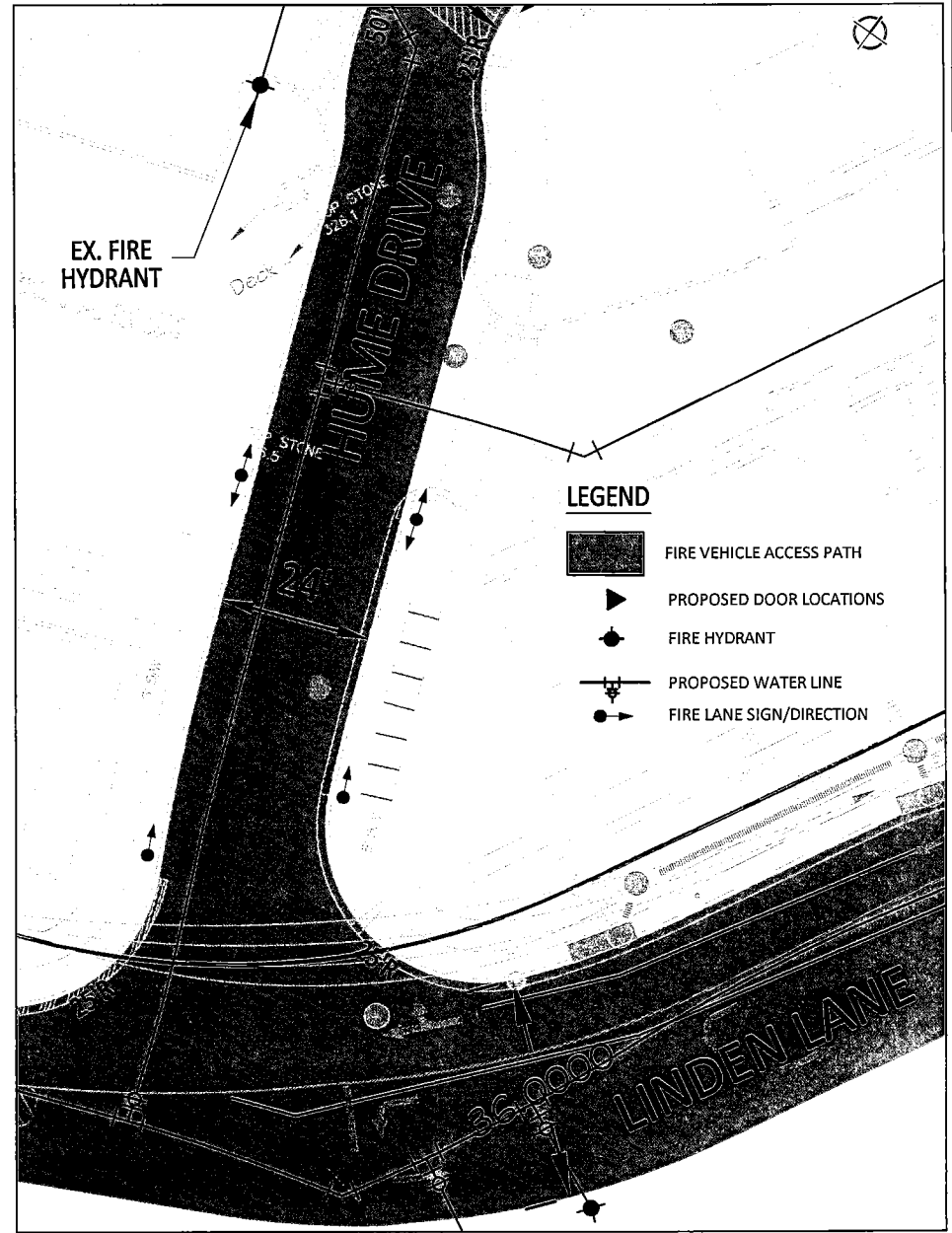
ENLARGEMENT D SCALE: 1"=30'
