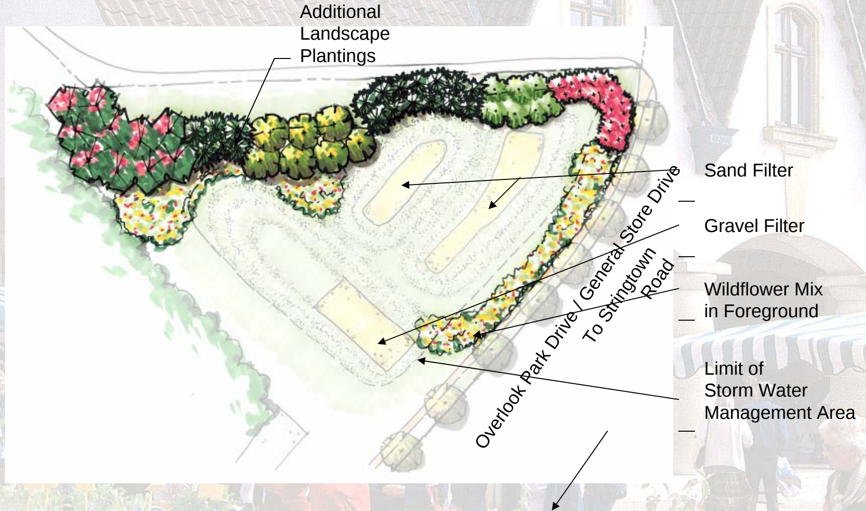
Concept for Storm Water Pond #2
