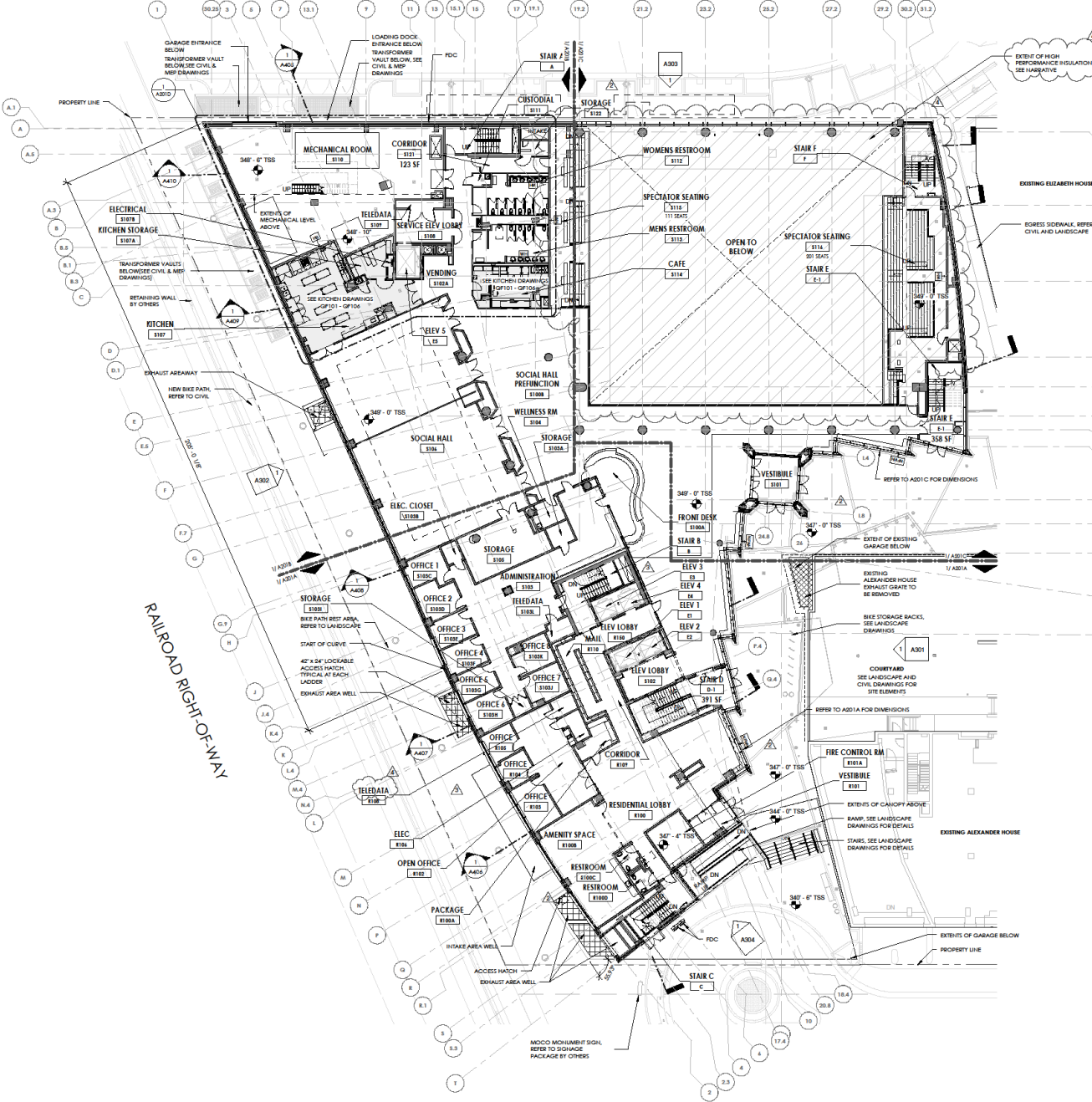
1 PLAZA LEVEL FLOOR PLAN - OVERALL A001 SCALE: 1/16" = 1'-0"
